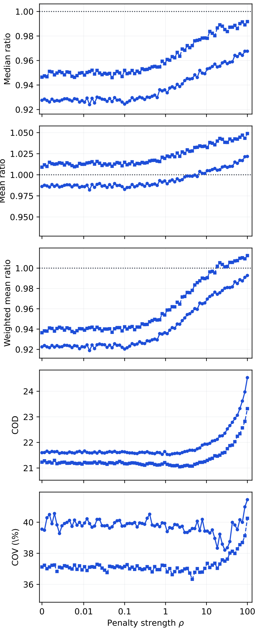
Direct
