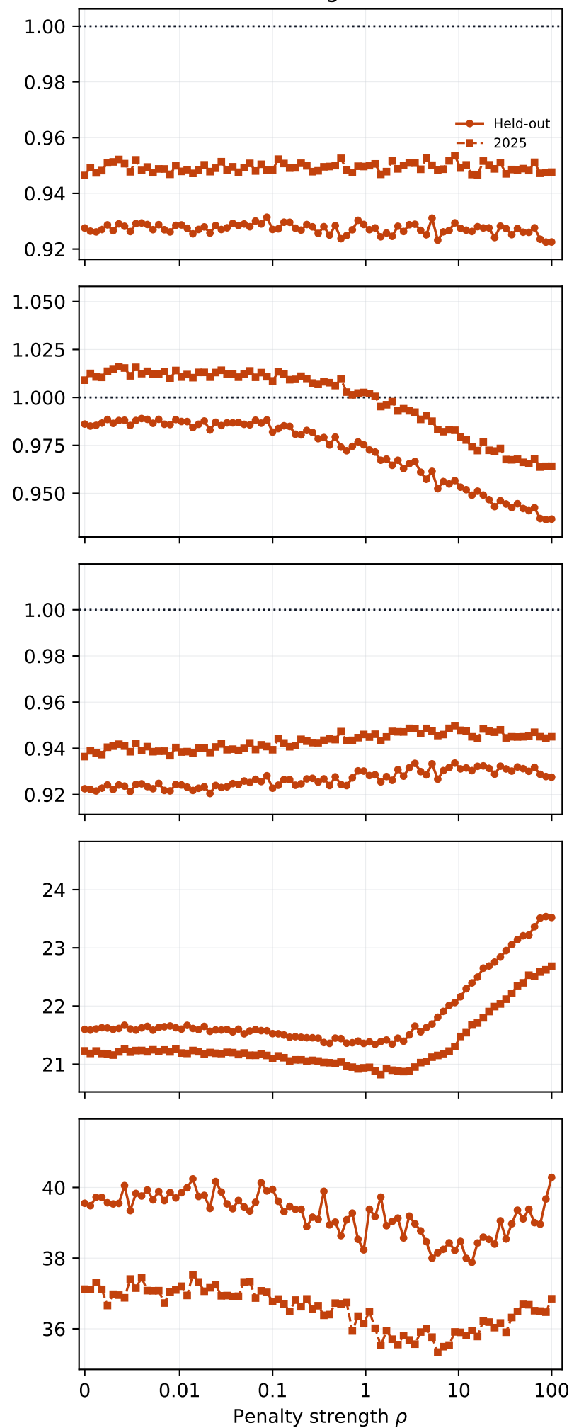
Surrogate
