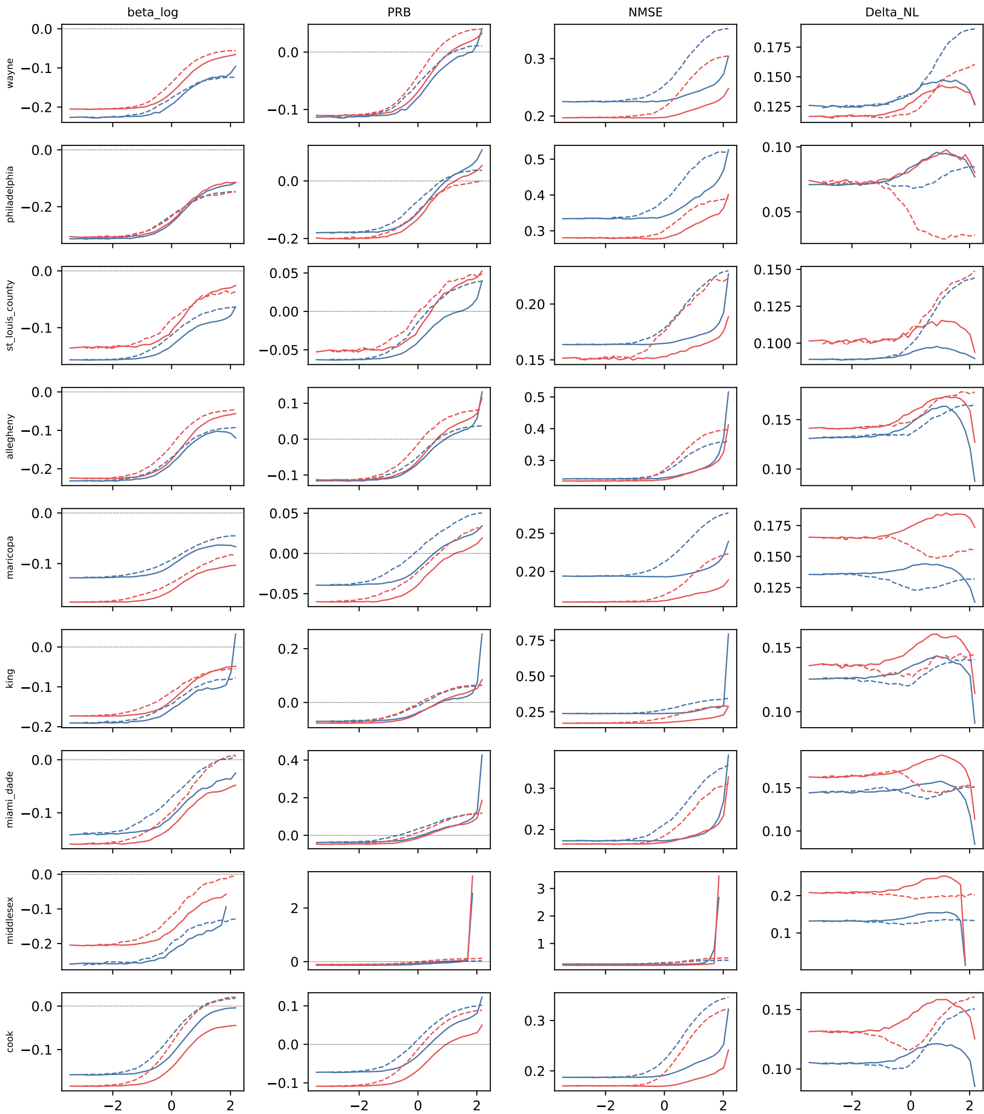
Nine-jurisdiction key paths (solid Direct, dashed Surrogate; blue CV, red 2025)
