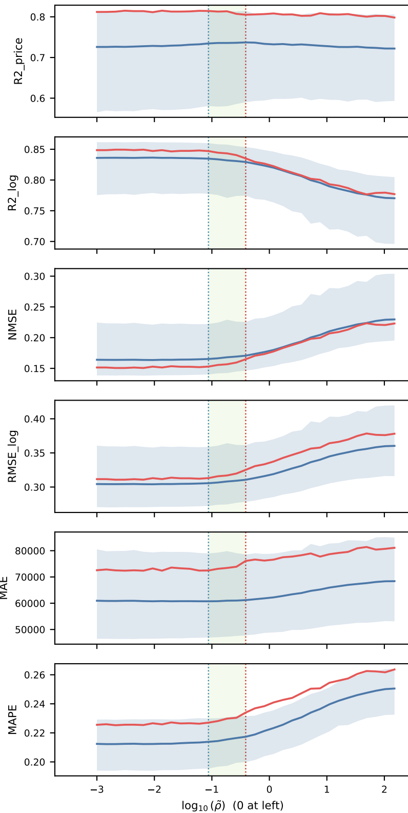
Surrogate
