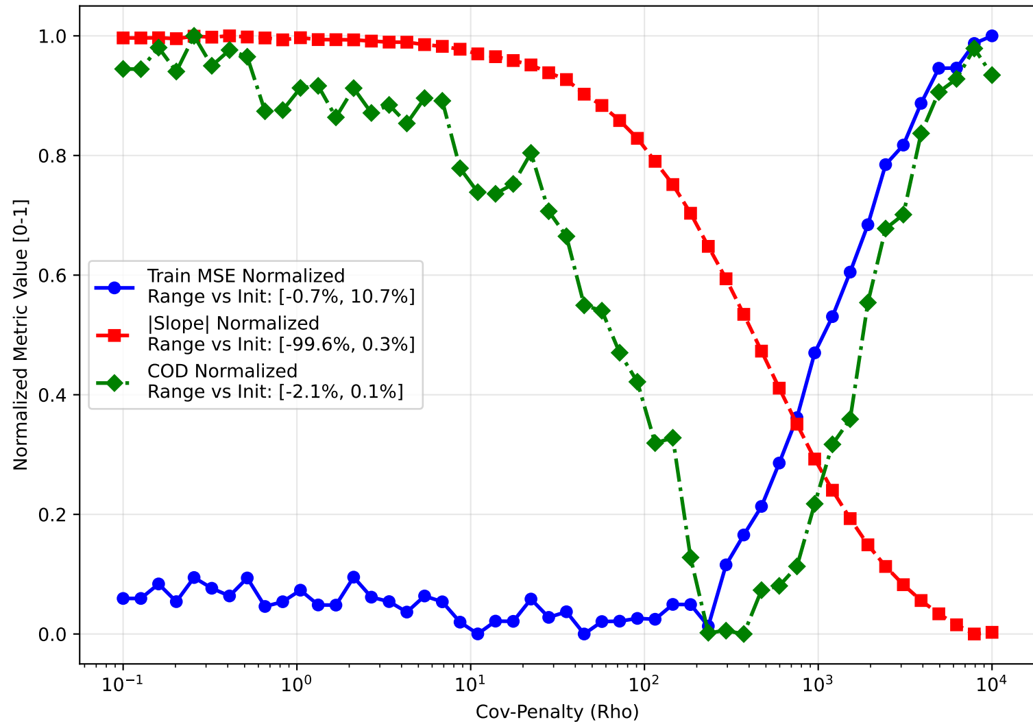
TRAIN Set: Metrics vs Cov-Penalty (Normalized)
