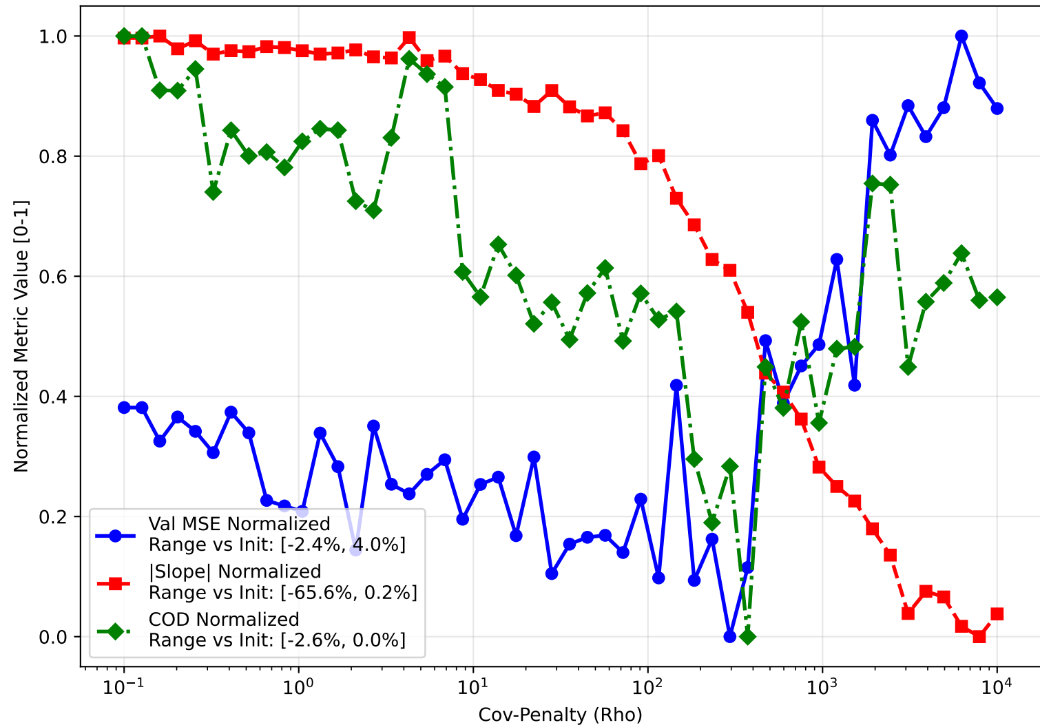
VALIDATION Set: Metrics vs Cov-Penalty (Normalized)
