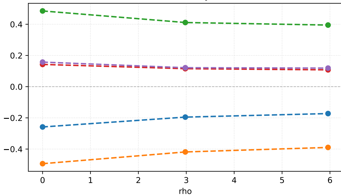
LGBCovPenalty[diff]
