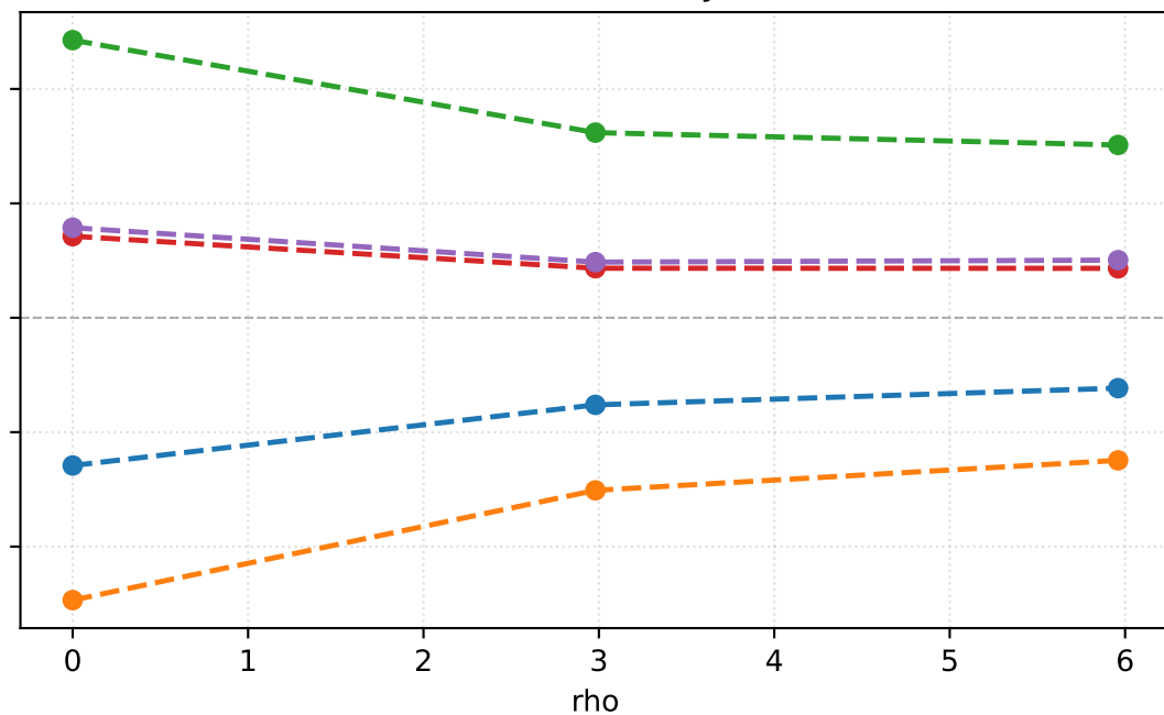
LGBSmoothPenalty[diff]
