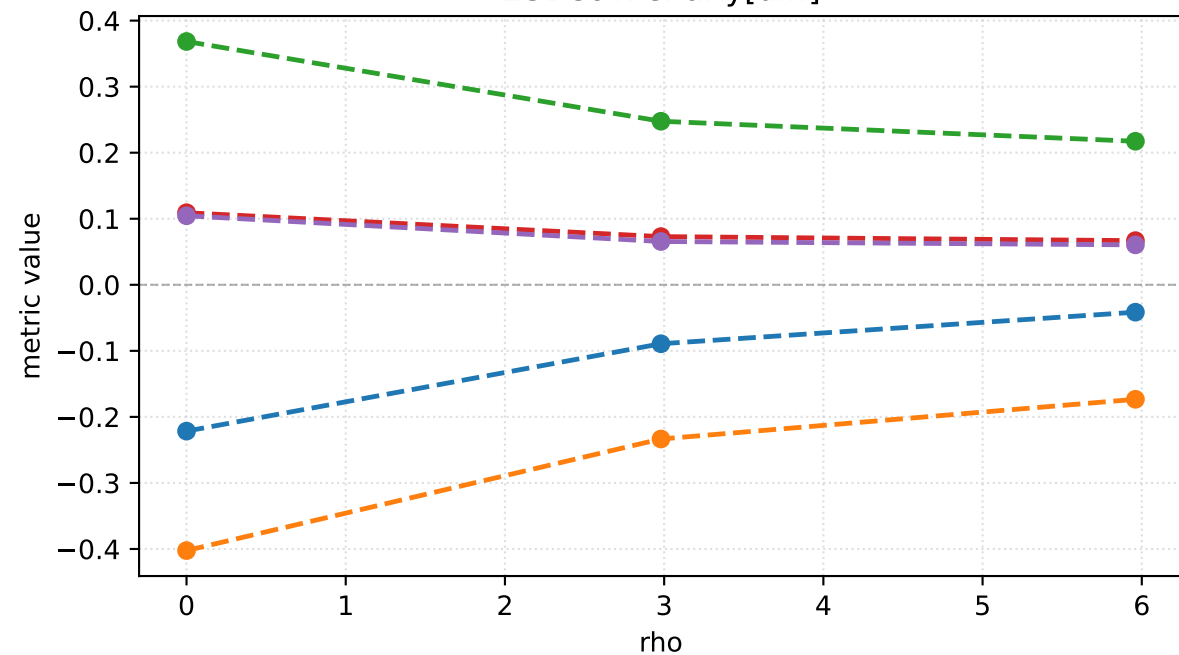
LGBCovPenalty[diff]
