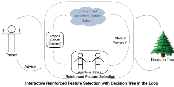
Fig. 1. Interactive reinforced feature selection via interaction with external trainers and downstream tasks (decision tree).
