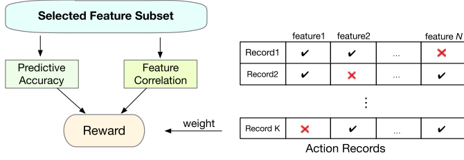
Fig. 8. General process of measuring reward with historical action records.
