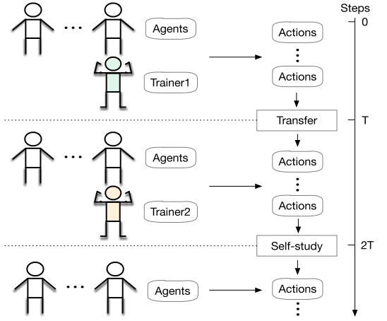
Fig. 4. General process of Hybrid Teaching strategy. One trainer gives advice first; then, another trainer gives advice. Finally, agents explore and learn by themselves.
