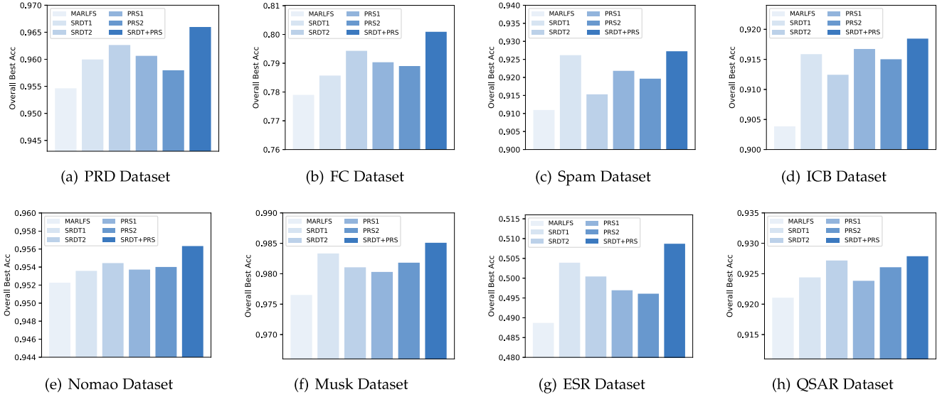
Fig. 11. Best Acc comparison of variant methods.
