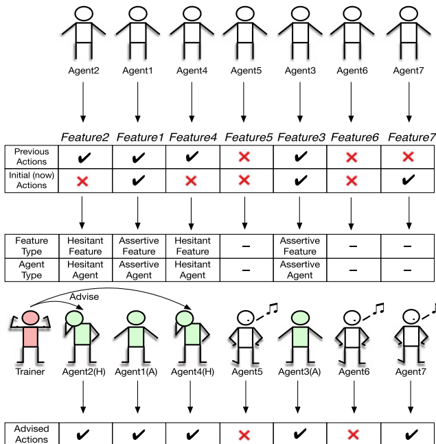
Fig. 3. General process of trainer guiding agents. Our framework first identifies assertive agents (labeled by 'A') and hesitant agents (labeled by 'H'). Then, the trainer offers advice to hesitant agents.
