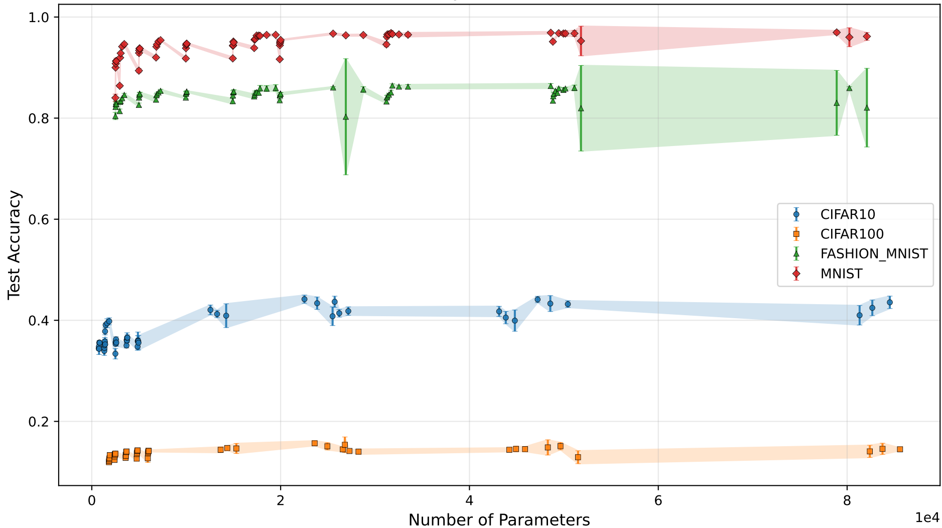
GTN Test Accuracy vs Number of Parameters
