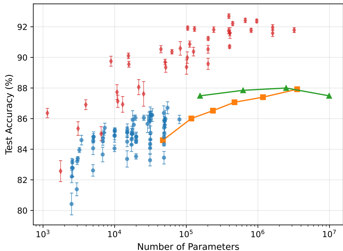
Fashion-MNIST
