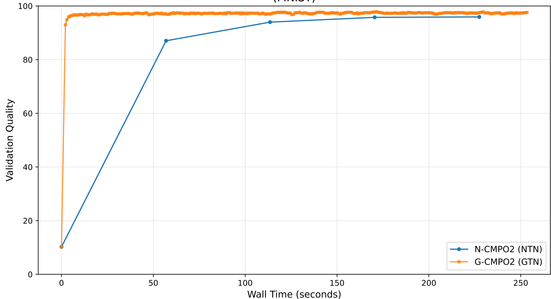
N-CMPO2 vs G-CMPO2: Validation Quality vs Wall Time (MNIST)
