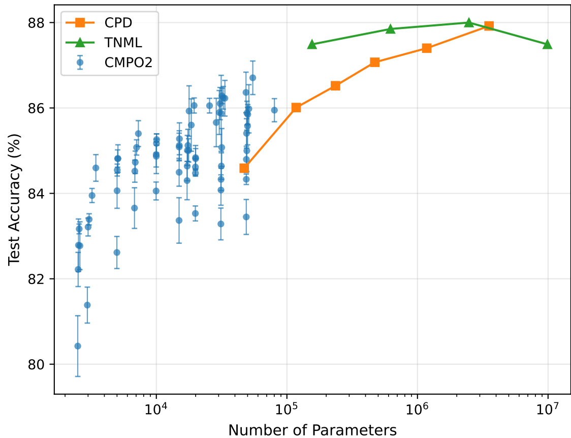
Fashion-MNIST
