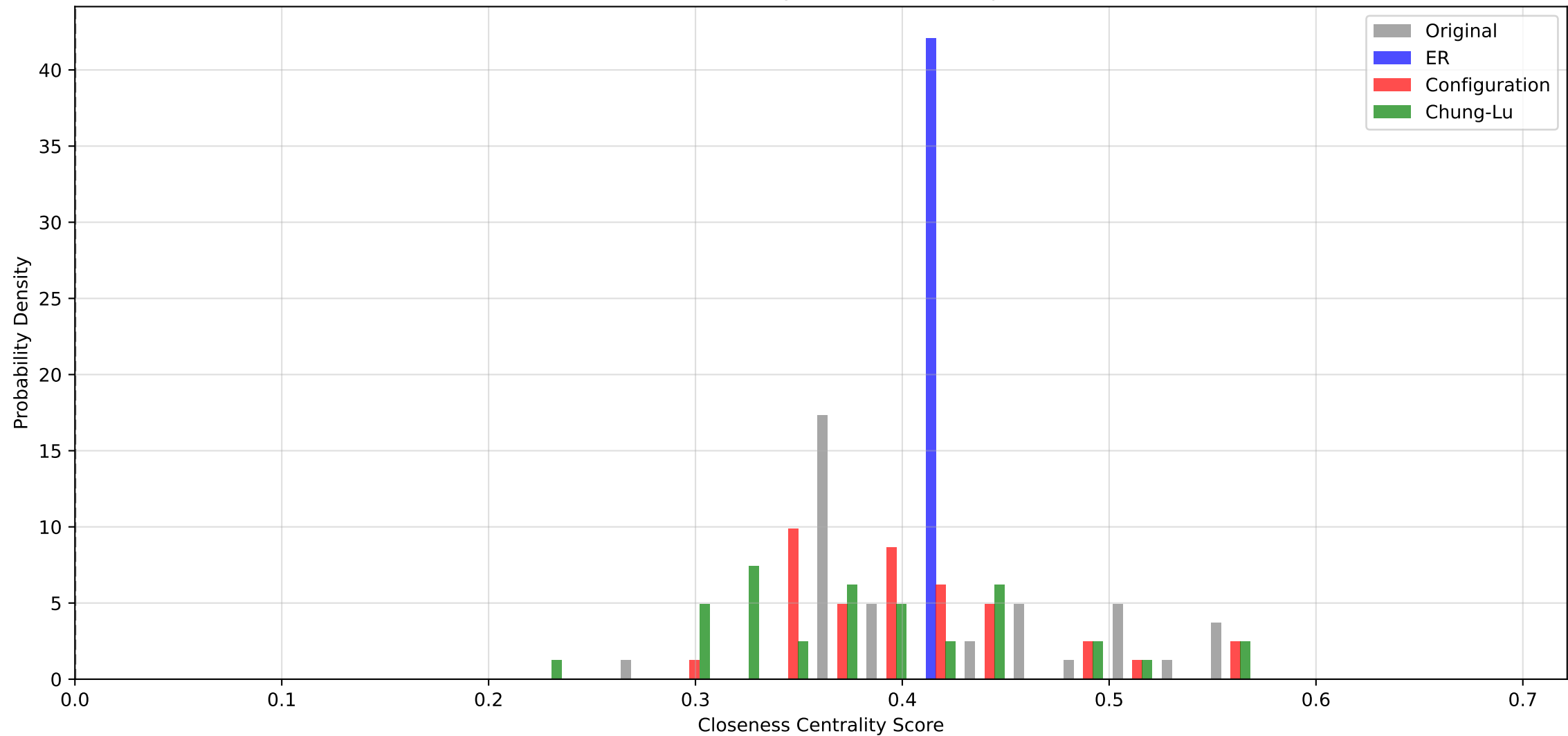
Closeness Centrality Distribution Comparison
