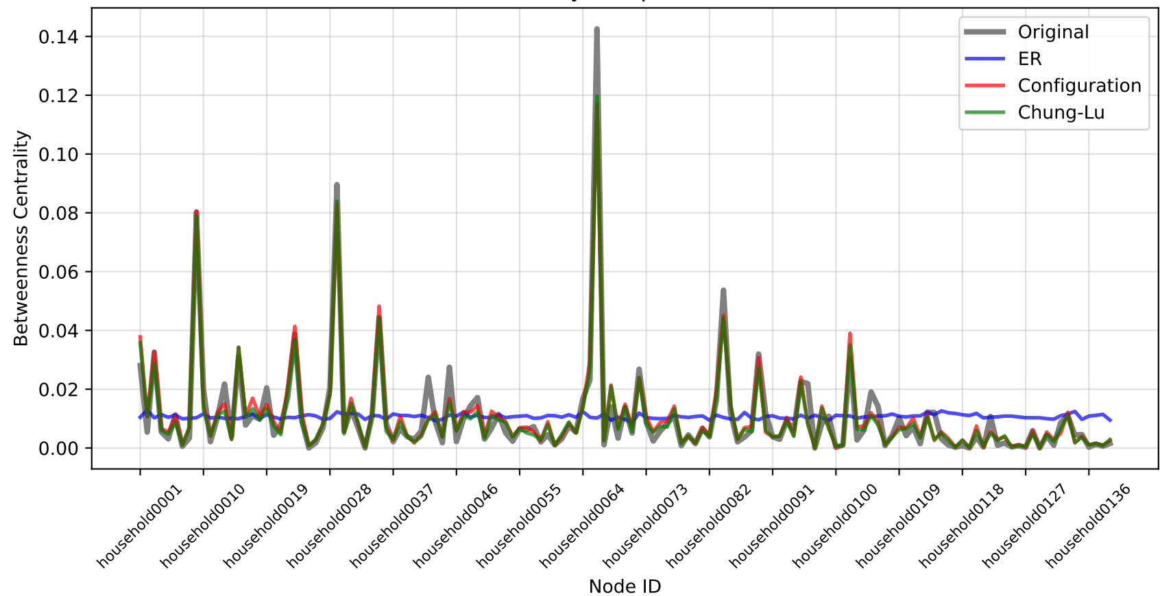
Betweenness Centrality Comparison (ensemble = 100)
