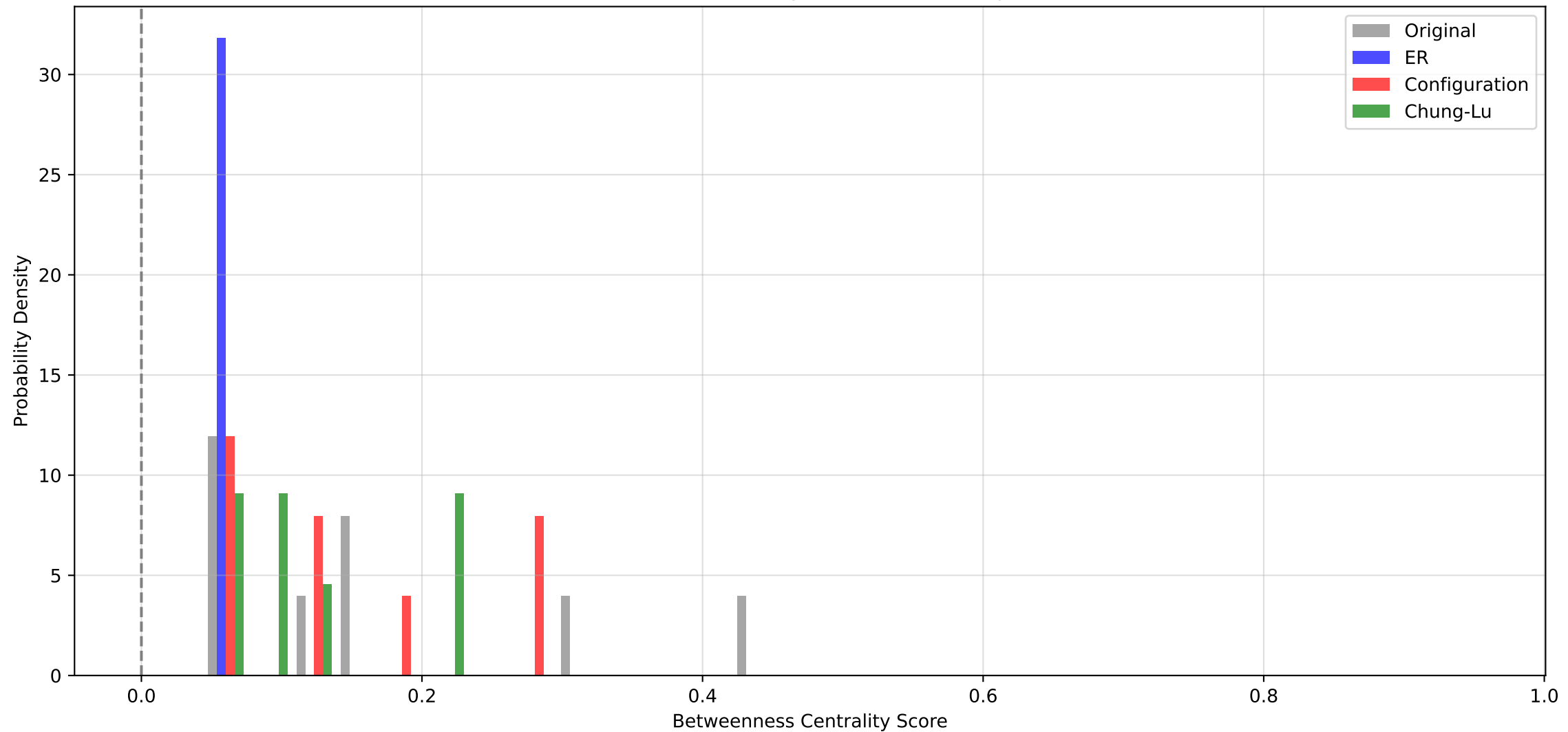
Betweenness Centrality Distribution Comparison
