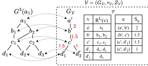
Figure 3: A illustration of View-based Inference. The inference for test node a_1 in N^L(a_1) is “simulated” by a counterpart for a' that 3-bisimilar to a_1 in a GMV, for GNN class \mathcal{M}^3 .
