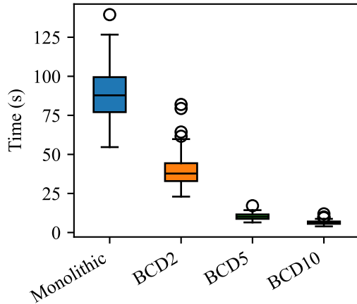
1000d Rosenbrock
