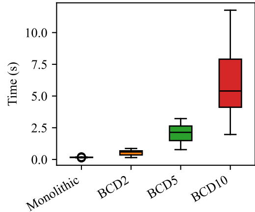
100d Rosenbrock
