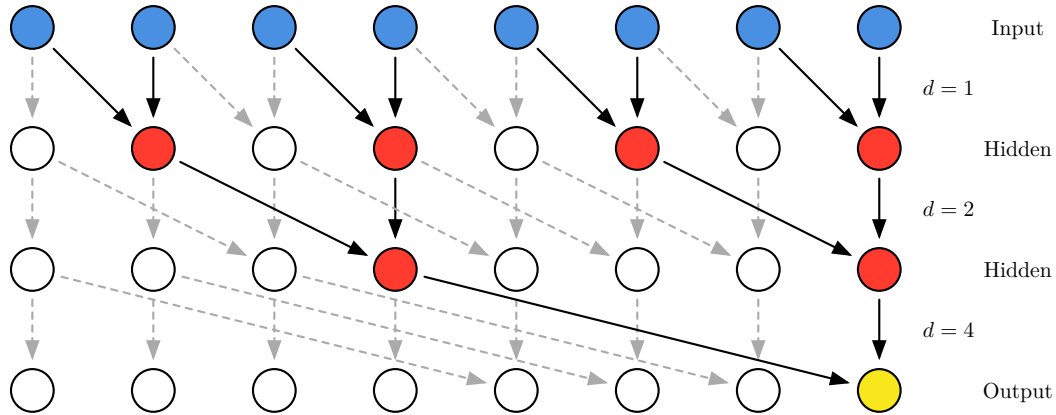
Figure 3: A dilated causal convolution with dilation factors d = 1, 2, 4 . Replicated from Lee et al. (2021).
