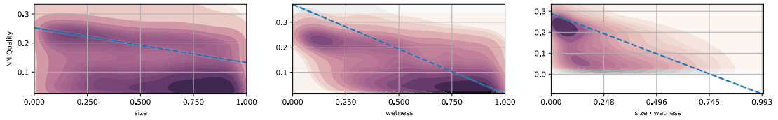
Figure 19: Quality score prediction analyzed over 16421 datapoints from test dataset (cf. Table 4), data between the 15th and 85th percentile is shown in color
