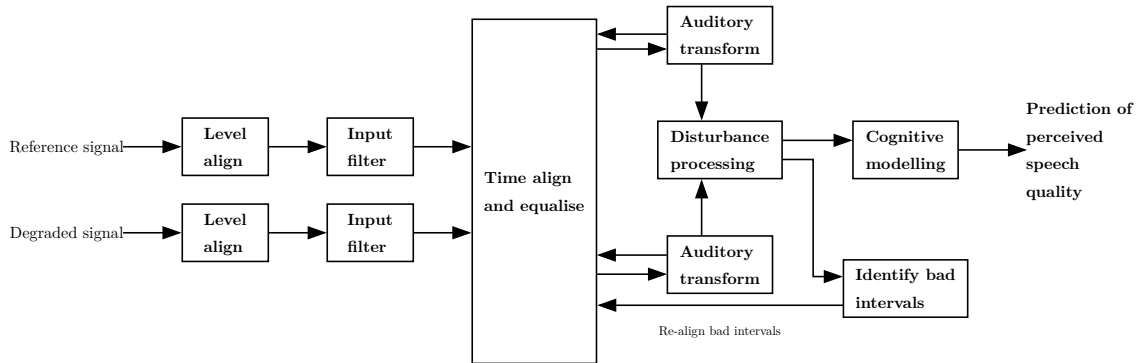
Figure 4: Structure of Perceptual Evaluation of Speech Quality (PESQ) model taken from Rix et al. (2001).
