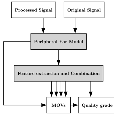
Figure 5: High-level representation of the Perceptual Evaluation of Audio Quality (PEAQ) model taken from Thiede et al. (2000).
