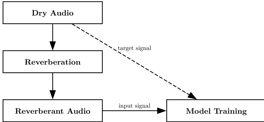
Figure 6: Dereverberation preprocessing pipeline
