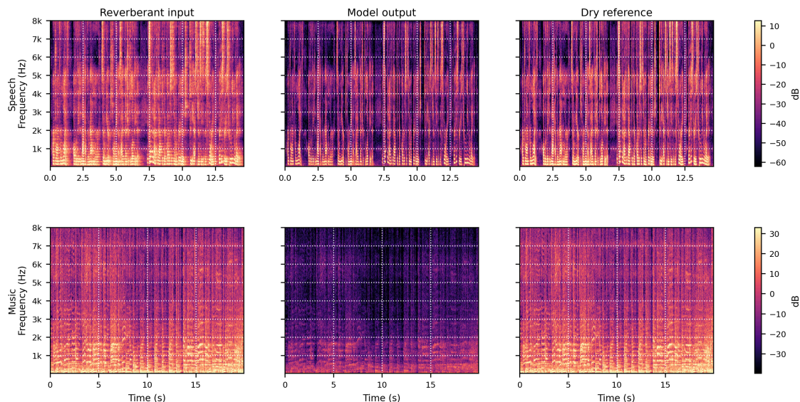
Figure 13: Spectrogram comparison of input (left) and output (middle) of StoRM on a speech (top) and music (bottom) sample.
