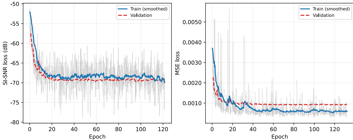
Figure 10: Training curves for Conv-TasNet with different loss functions. Smoothed using an exponential moving average with \alpha = 0.05 .
