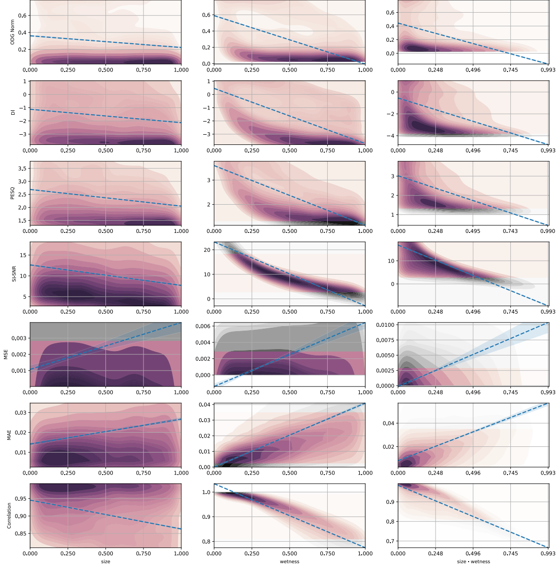
Figure 9: Metrics usable as loss functions analyzed over 16421 datapoints from test dataset (cf. Table 4), data between the 15th and 85th percentile is shown in color
