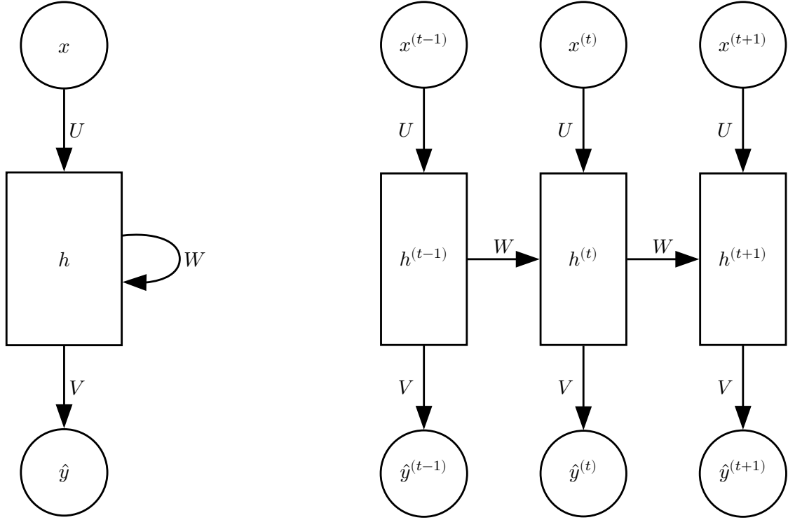
Figure 1: RNN architecture for an input sequence x , hidden connections parametrized by a weight matrix U and hidden-to-hidden recurrent connections parametrized by a weight matrix W . Shown on the right is the unrolled version of an RNN cell across three time steps. Replicated from Goodfellow et al. (2016).
