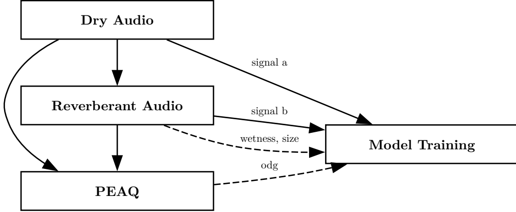
Figure 7: Perceptual loss preprocessing pipeline
