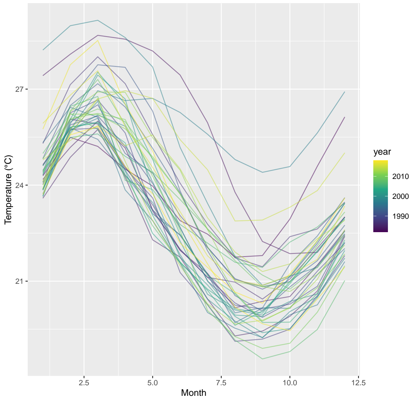
El Niño SST: Seasonal patterns across years
