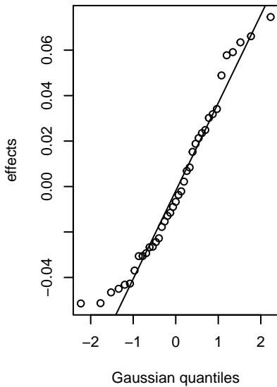
s(id,37.7)
