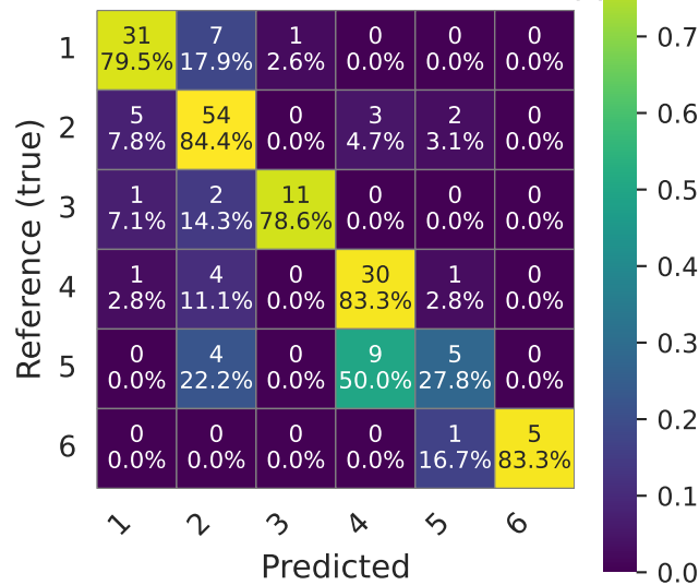
Confusion matrix (row-normalized). kappa = 0.690
