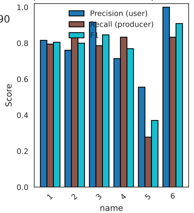
Per-class precision (user), recall (producer) and F1
