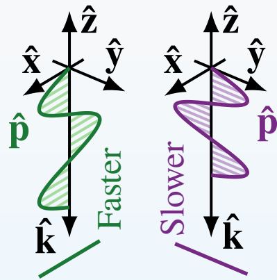
Eigenpolarized waves
