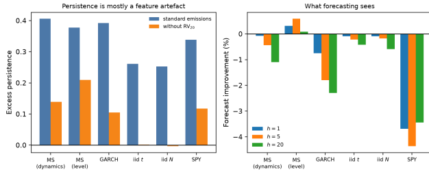
Figure 5: Left: apparent regime persistence, with the standard emission vector and with the 20-day rolling volatility removed. On i.i.d. data the first is large and the second is zero. Right: forecast improvement from conditioning on the inferred state. Only the right panel separates the worlds that contain regimes from those that do not.
