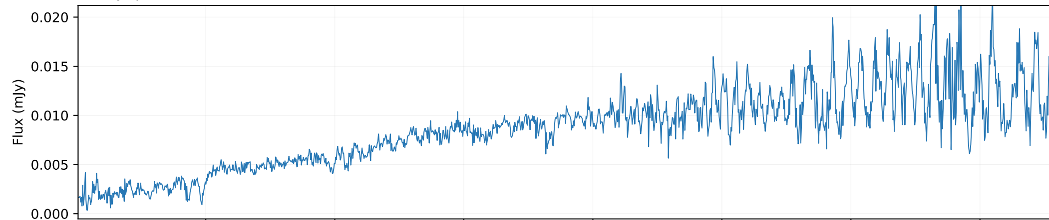
QSO spectrum × 0.1 (SDSS DR7Q)
