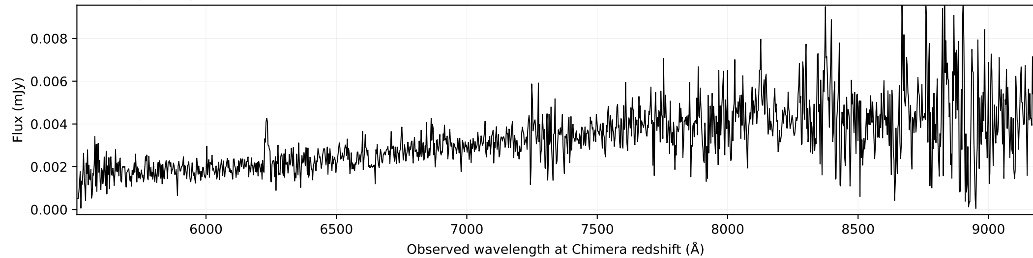
Safe composite spectrum
