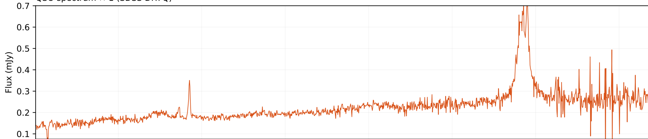
Safe composite spectrum
