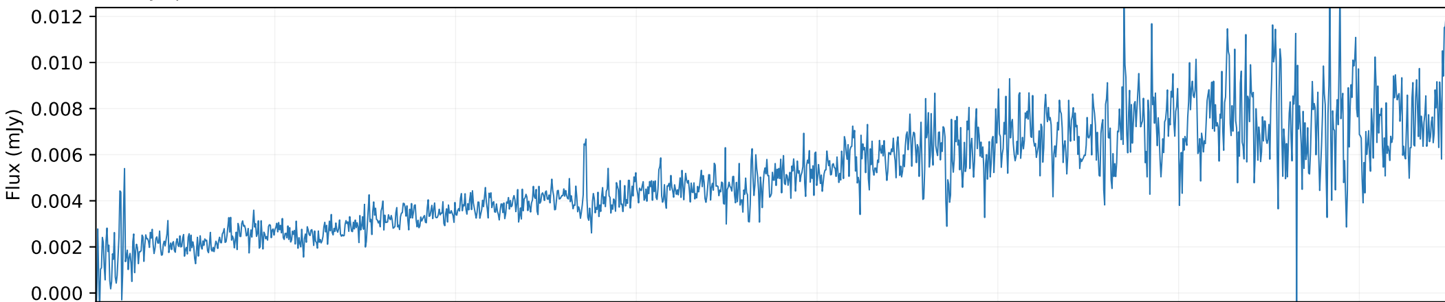
QSO spectrum × 0.3 (SDSS DR7Q)
