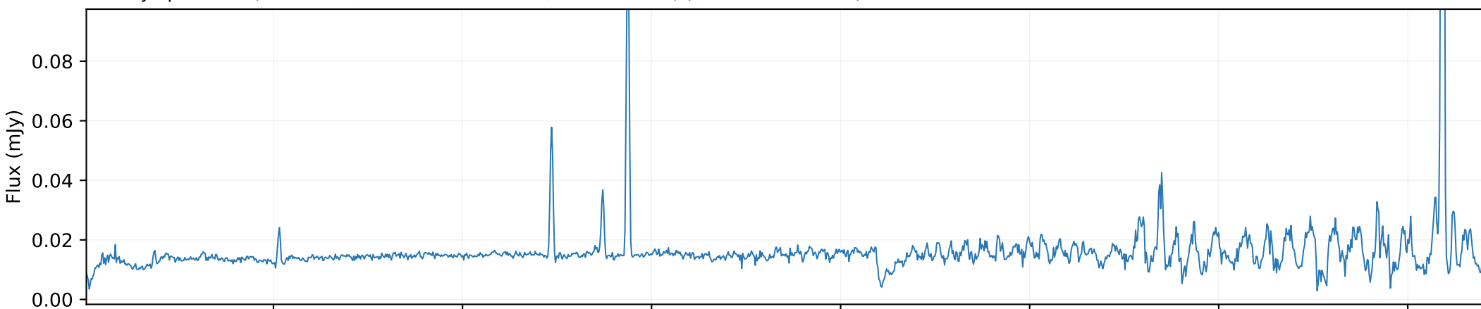
QSO spectrum × 0.0001 (SDSS DR7Q)
