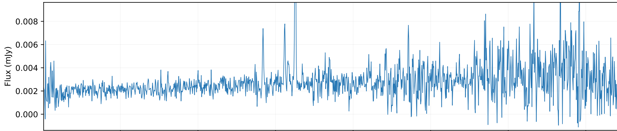
QSO spectrum \times 0.01 (SDSS DR7Q)
