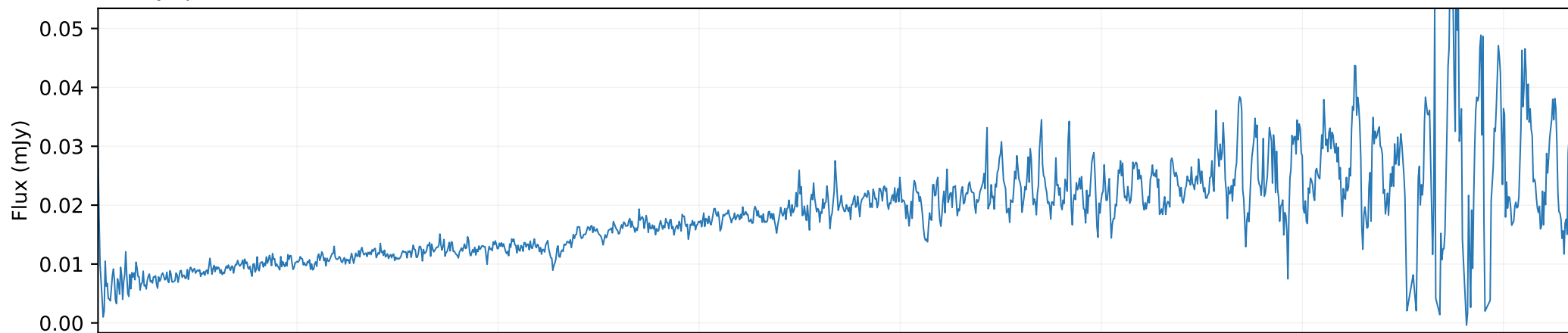
QSO spectrum × 0.003 (SDSS DR7Q)
