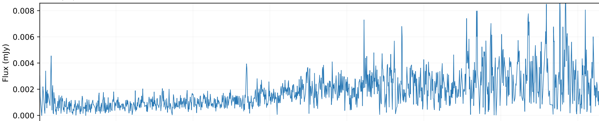
QSO spectrum × 0.0003 (SDSS DR7Q)
