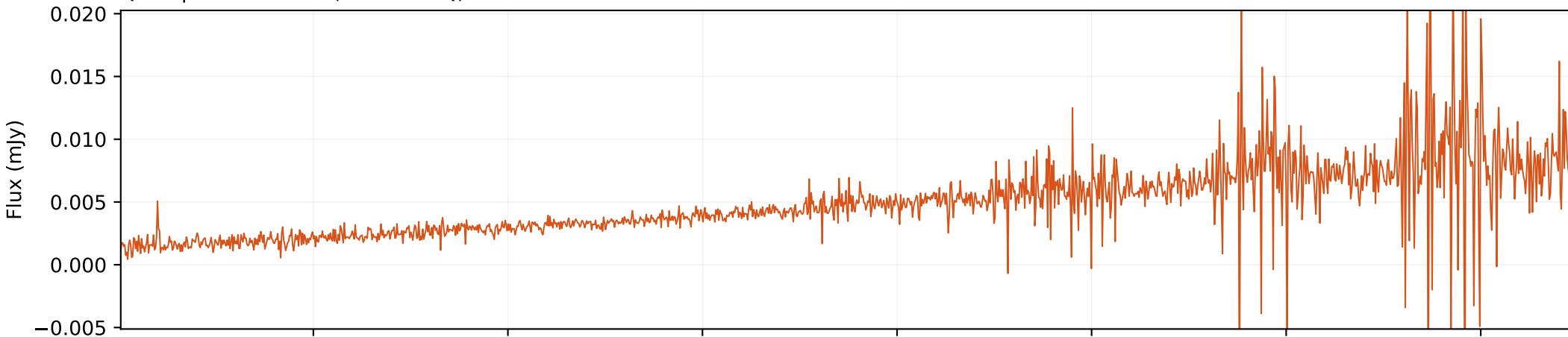
Safe composite spectrum
