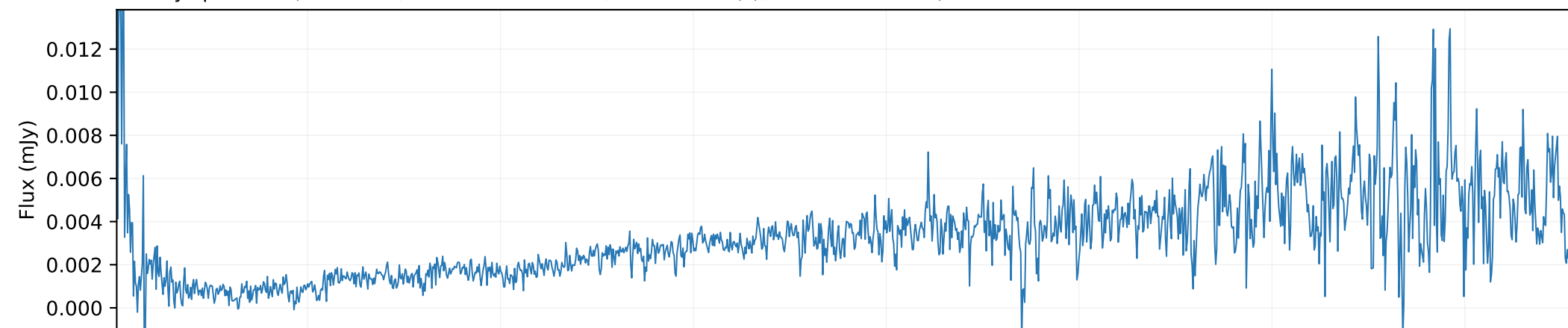
QSO spectrum \times 0.01 (SDSS DR7Q)
