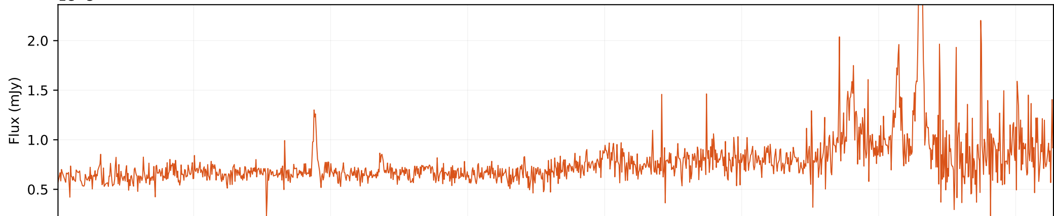
Safe composite spectrum
