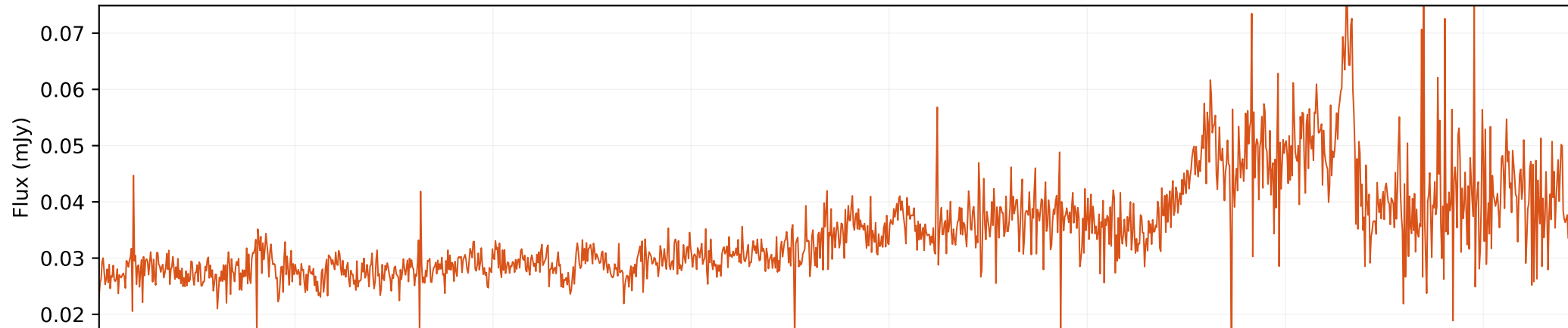
Safe composite spectrum
