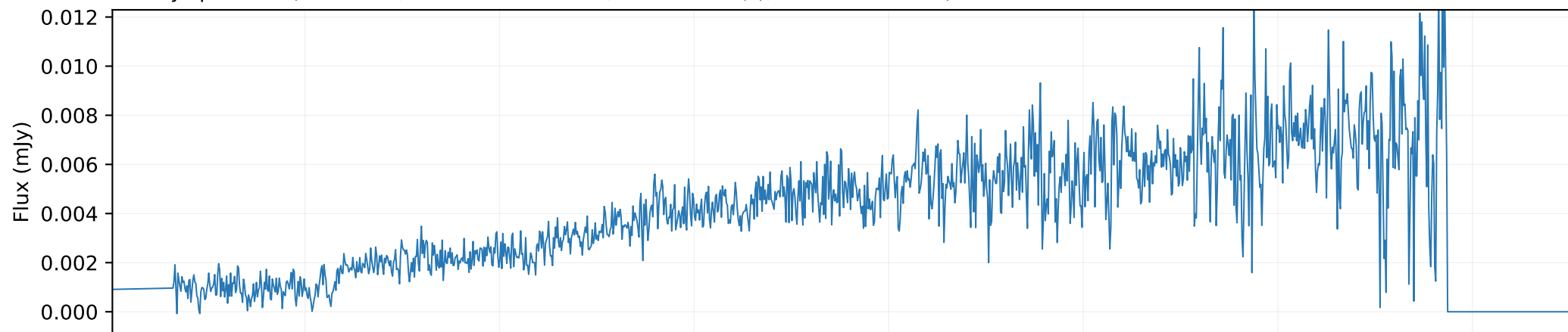
QSO spectrum × 0.001 (SDSS DR7Q)
