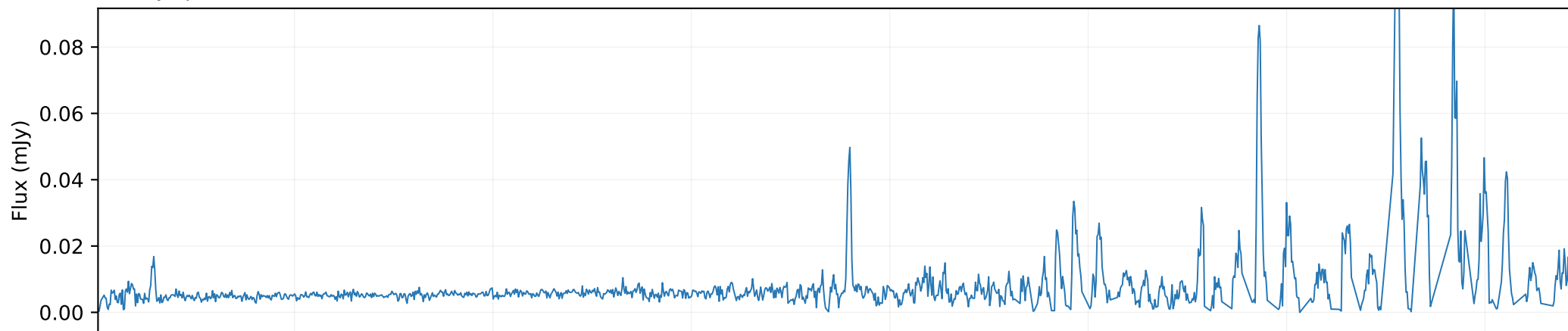
QSO spectrum \times 0.0001 (SDSS DR7Q)
