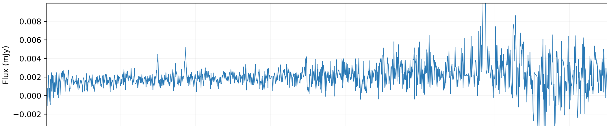
QSO spectrum \times 0.03 (SDSS DR7Q)
