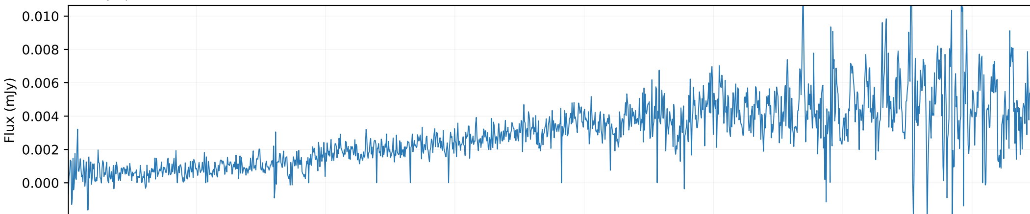
QSO spectrum \times 1 (SDSS DR7Q)
