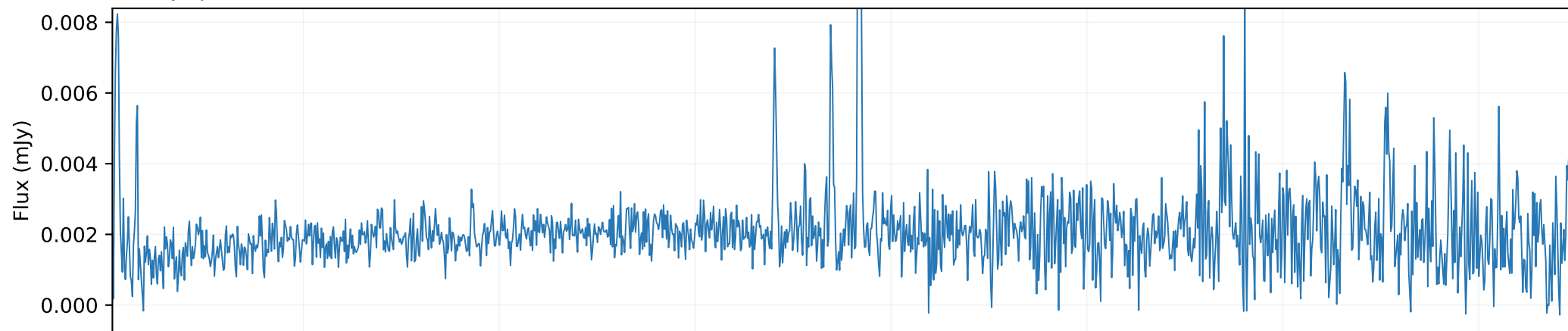
QSO spectrum \times 0.001 (SDSS DR7Q)
