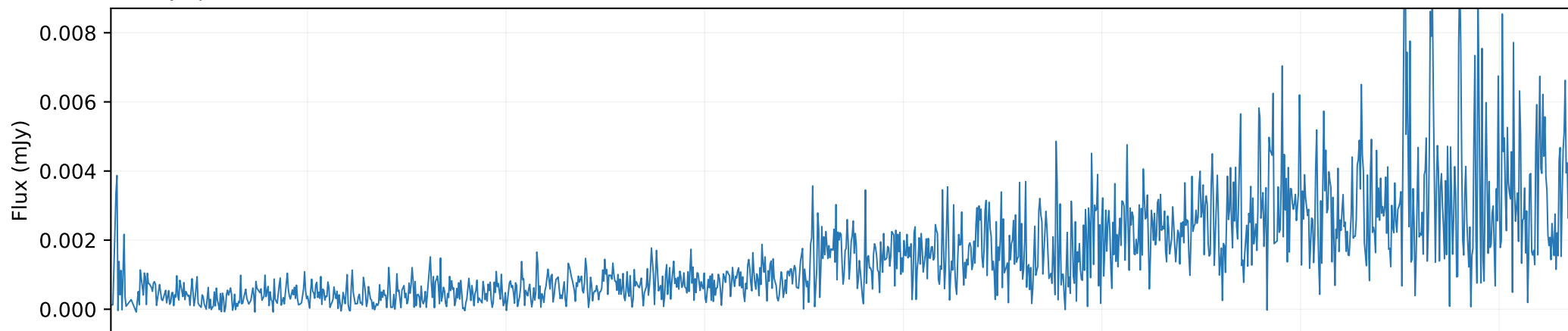
QSO spectrum × 0.0003 (SDSS DR7Q)
