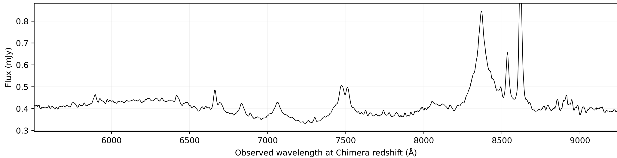
Safe composite spectrum
