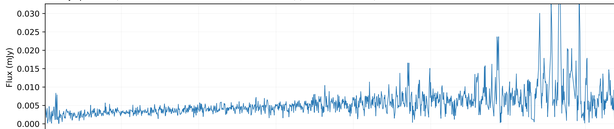
QSO spectrum \times 0.0003 (SDSS DR7Q)
