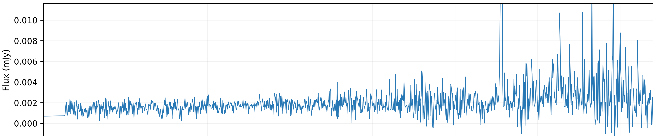
QSO spectrum \times 0.1 (SDSS DR7Q)
