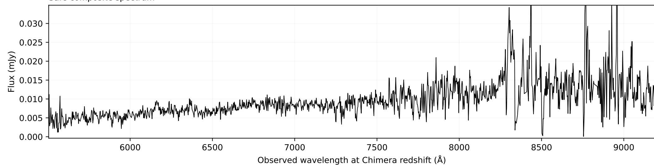
Safe composite spectrum
