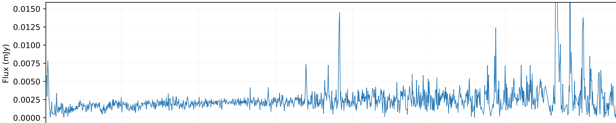
QSO spectrum \times 0.0001 (SDSS DR7Q)
