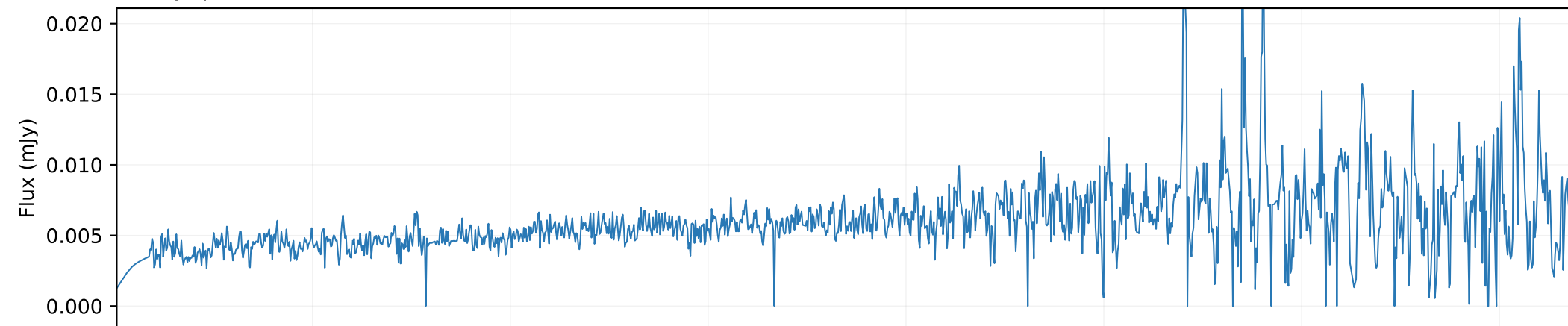
QSO spectrum × 0.0003 (SDSS DR7Q)
