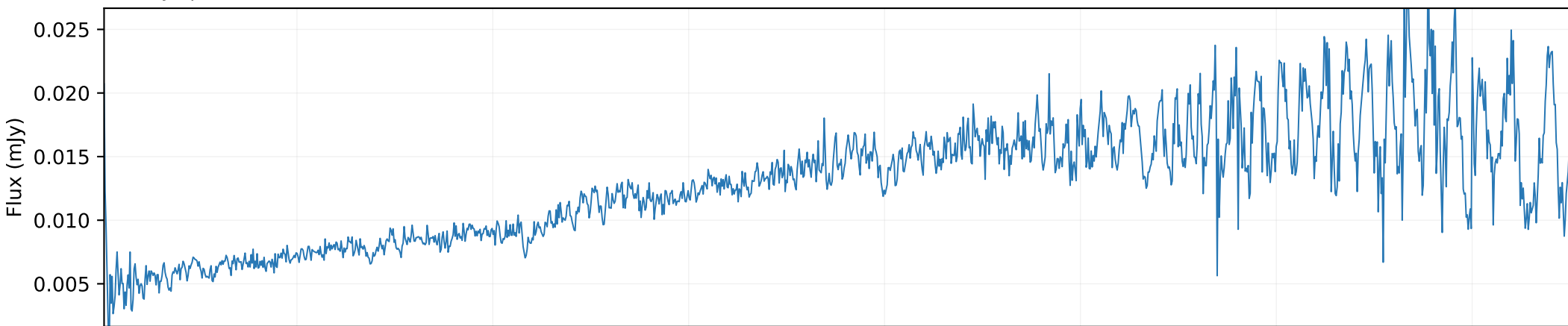
QSO spectrum × 0.01 (SDSS DR7Q)
