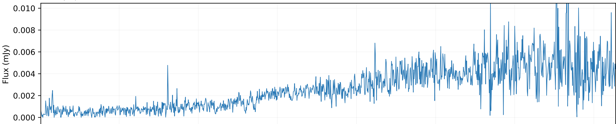
QSO spectrum × 0.0001 (SDSS DR7Q)
