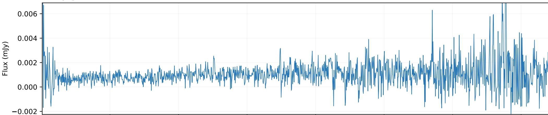
QSO spectrum × 0.03 (SDSS DR7Q)
