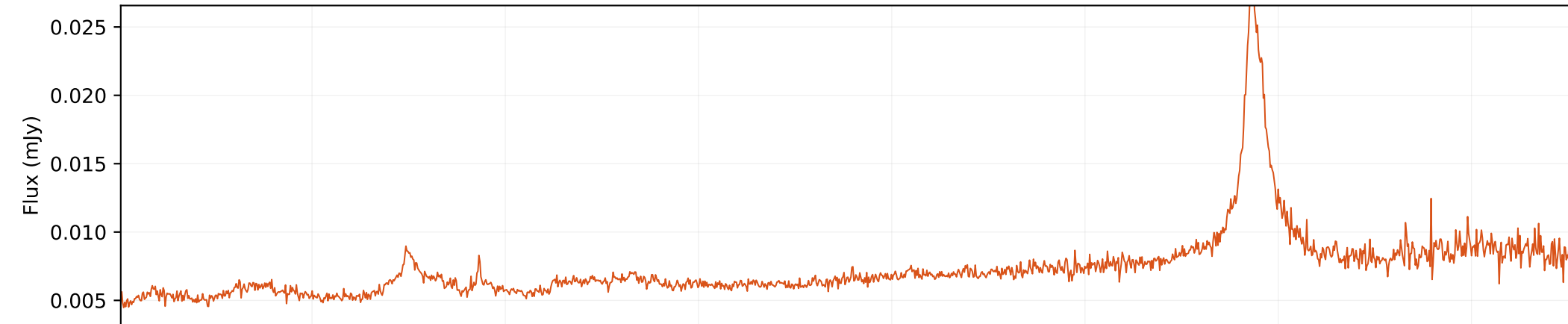
Safe composite spectrum
