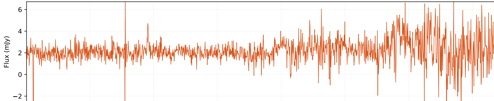
Safe composite spectrum
