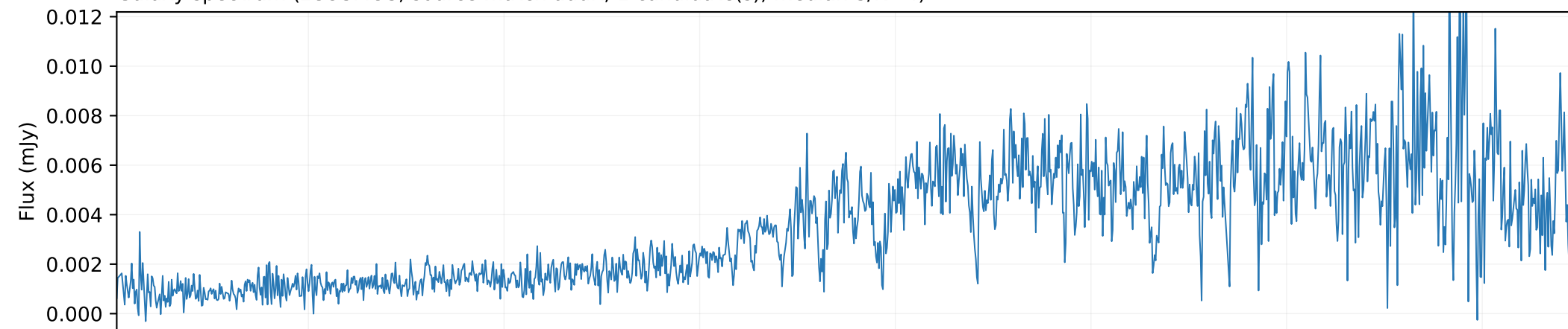
QSO spectrum × 0.003 (SDSS DR7Q)
