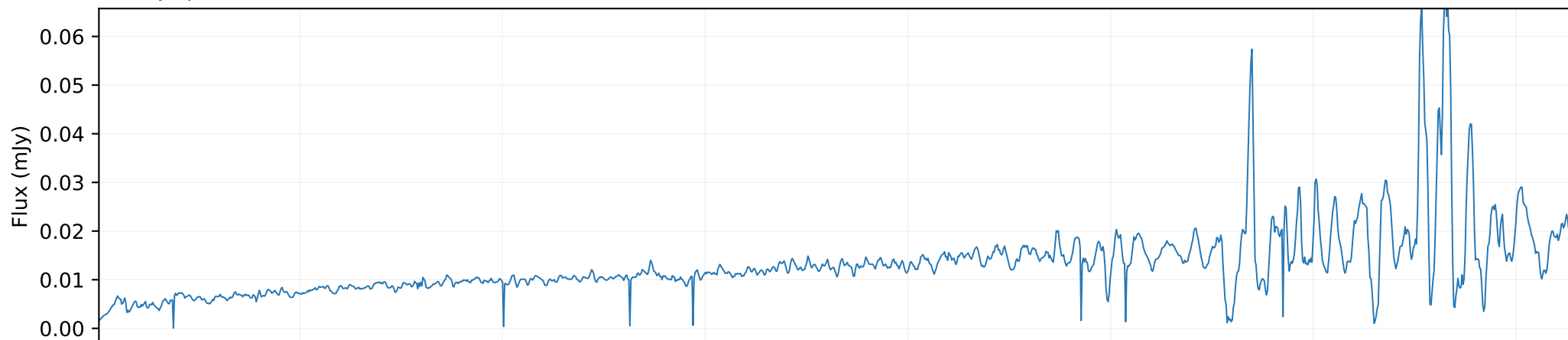
QSO spectrum × 0.0001
