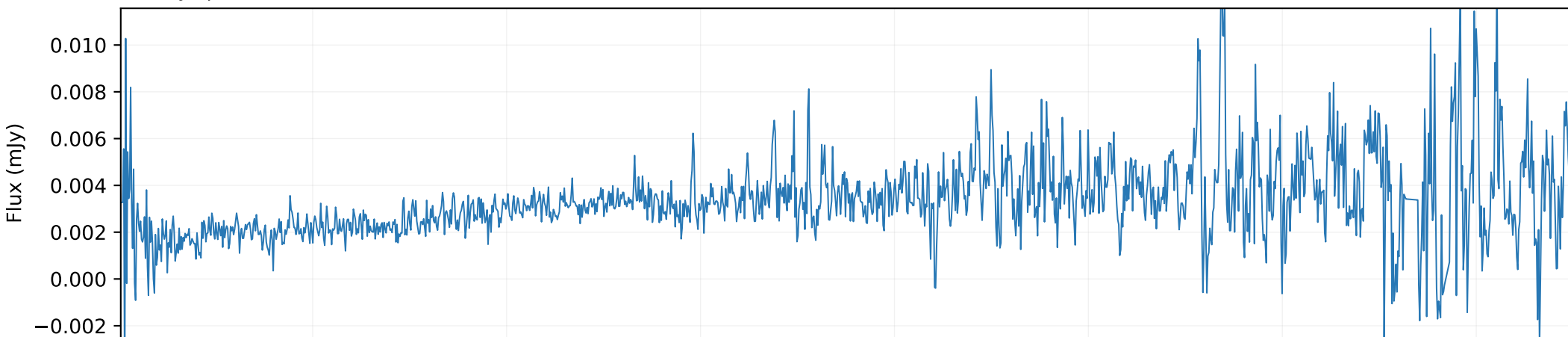
QSO spectrum × 0.1
