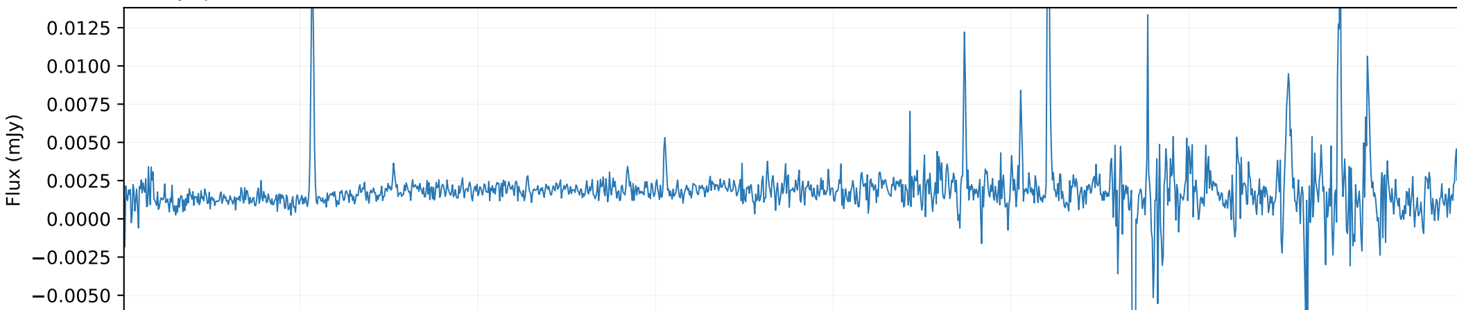
QSO spectrum × 0.1
