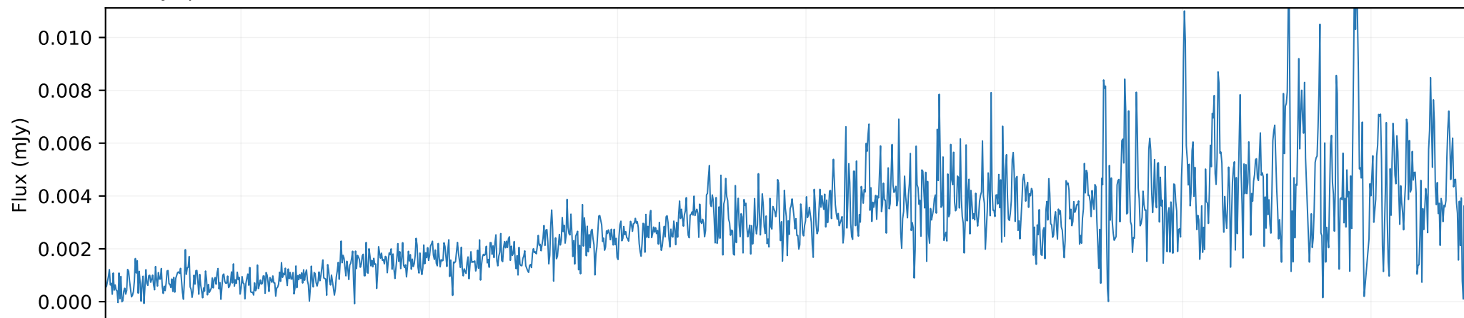
QSO spectrum × 0.001
