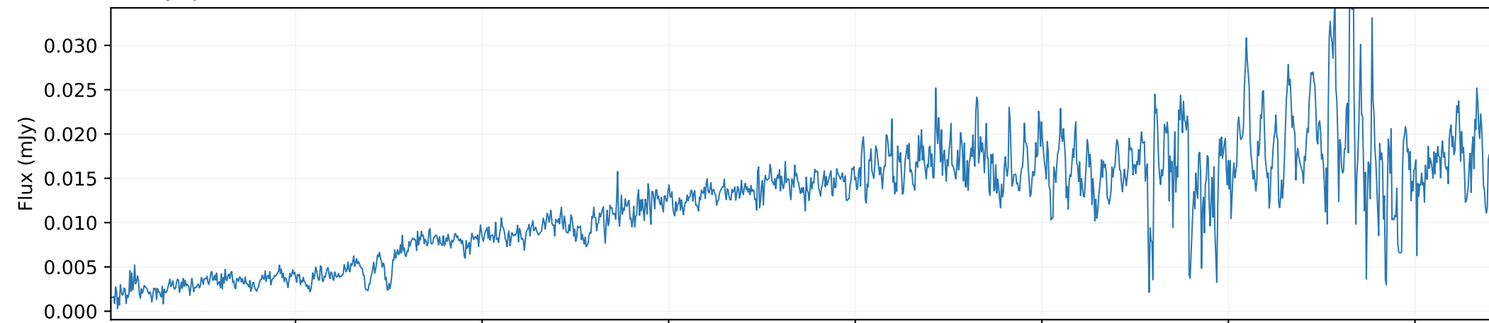
QSO spectrum × 0.01
