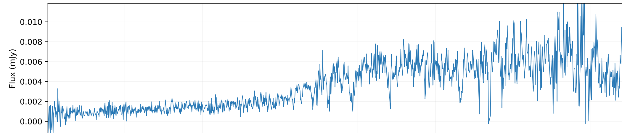
QSO spectrum \times 0.1
