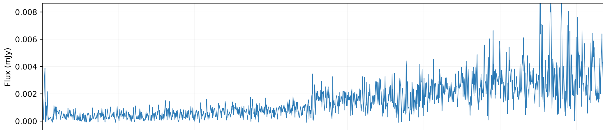
QSO spectrum × 0.0003
