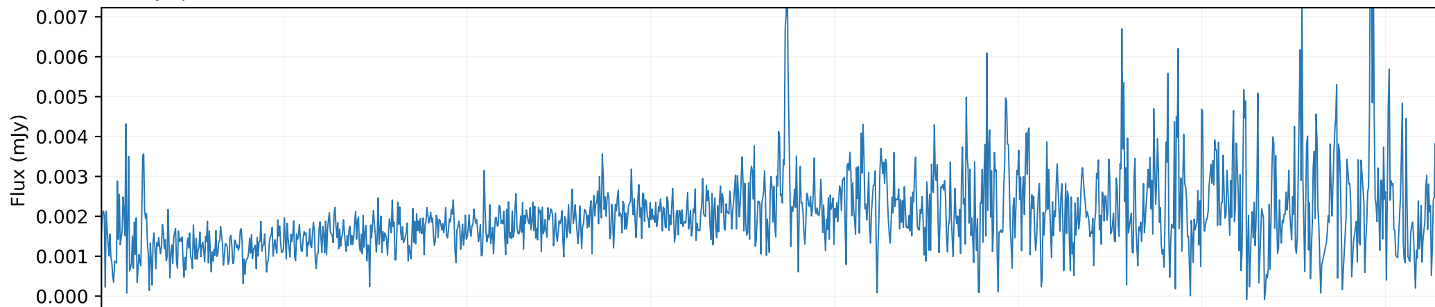
QSO spectrum \times 0.0001
