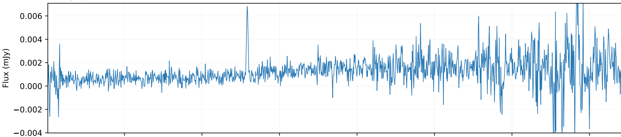
QSO spectrum × 1
