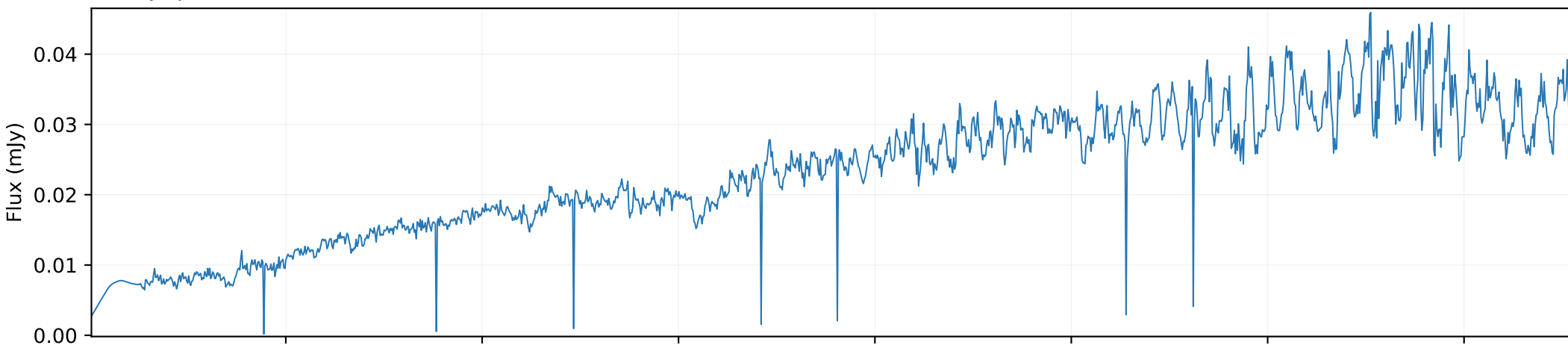
QSO spectrum × 0.3
