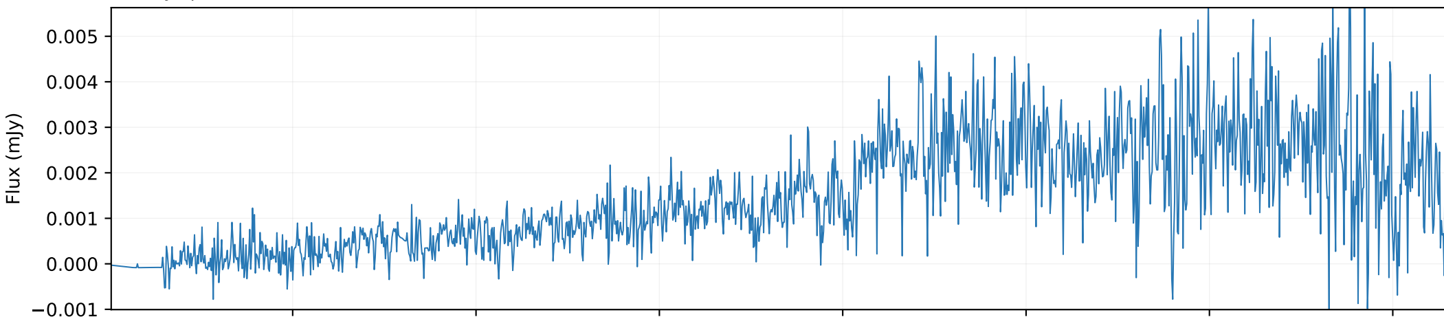
QSO spectrum × 0.003
