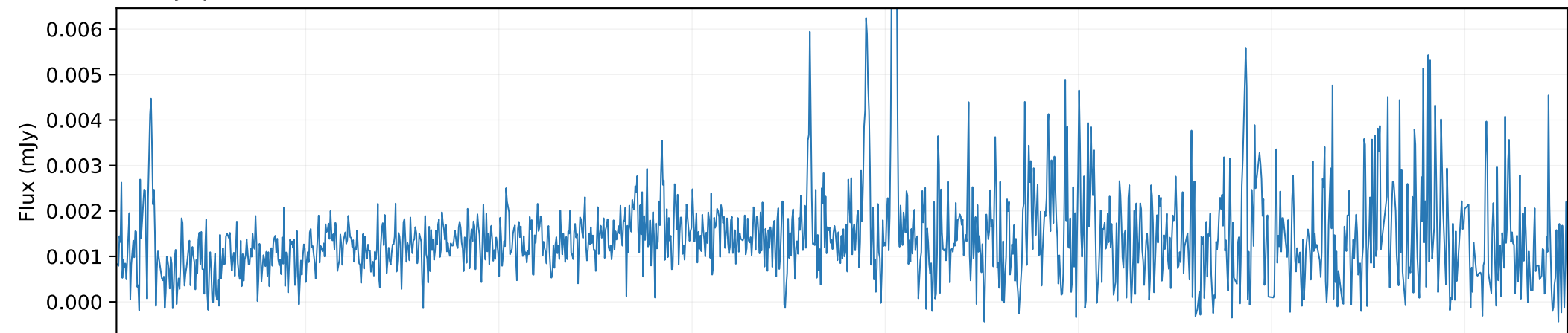
QSO spectrum × 0.003
