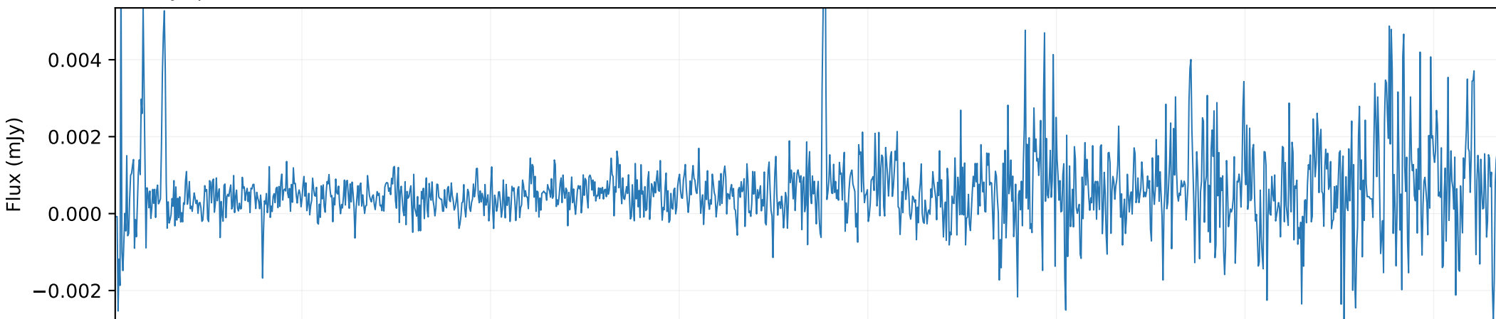
QSO spectrum × 0.03
