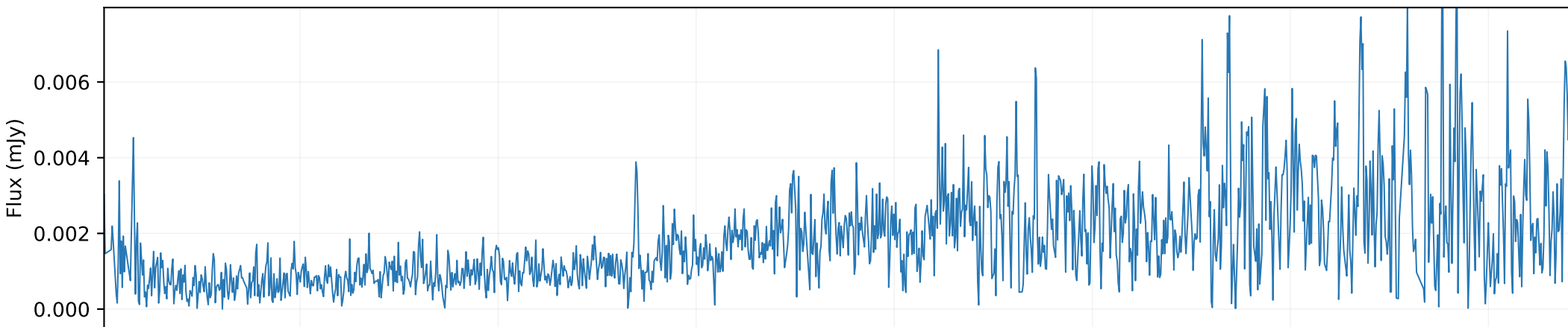
QSO spectrum × 0.0001
