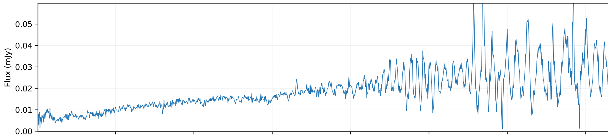
QSO spectrum × 0.003
