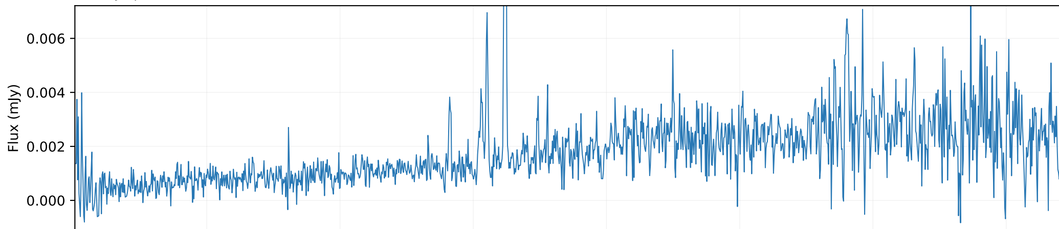
QSO spectrum × 0.01
