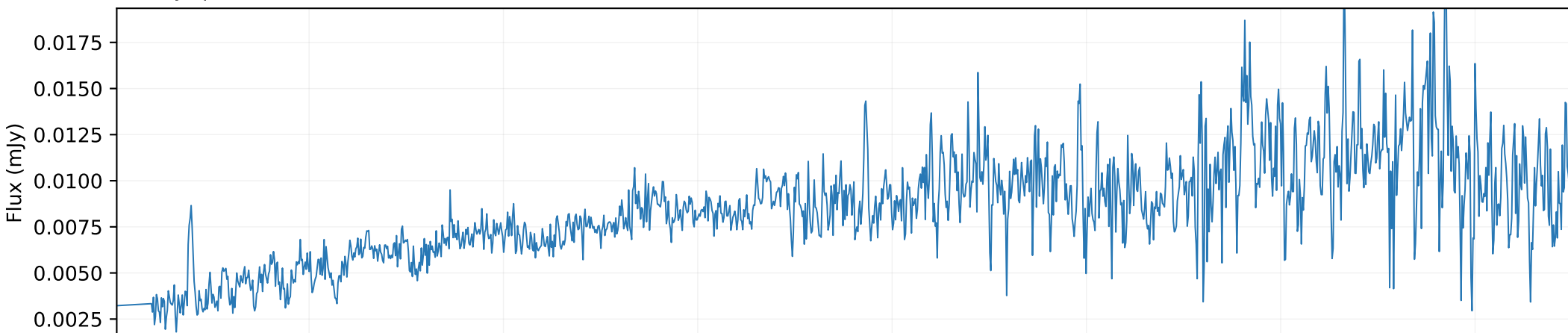
QSO spectrum × 1
