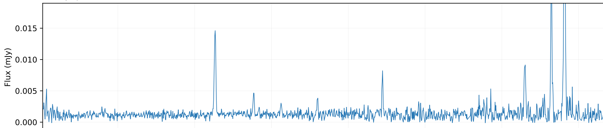
QSO spectrum × 0.003
