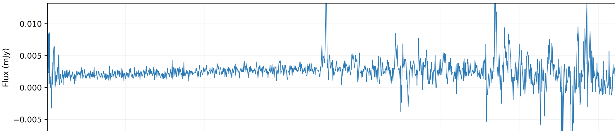
QSO spectrum × 0.3
