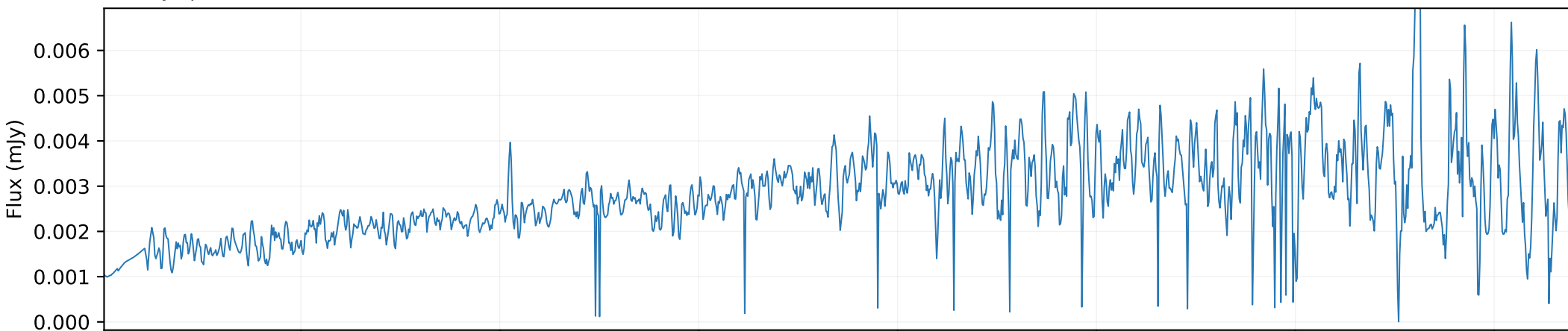
QSO spectrum × 0.0001
