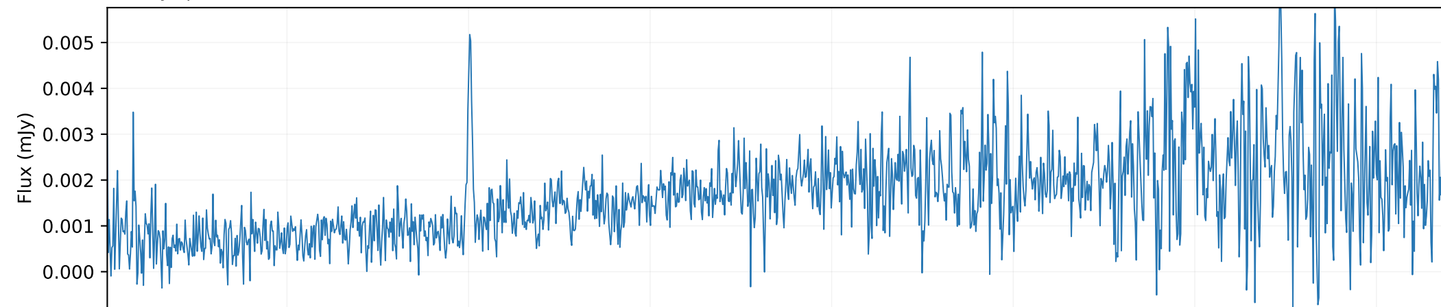
QSO spectrum × 0.01
