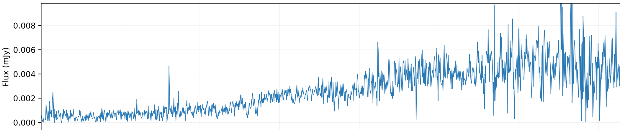
QSO spectrum \times 0.0001
