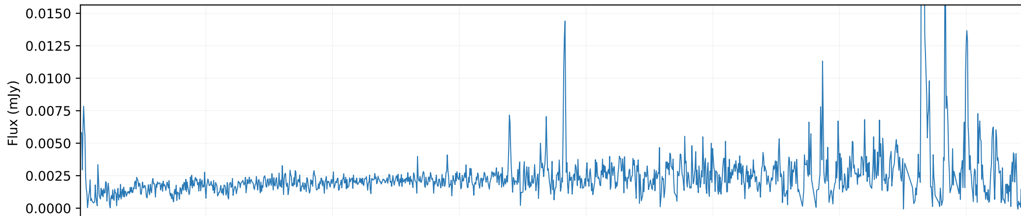
QSO spectrum \times 0.001
