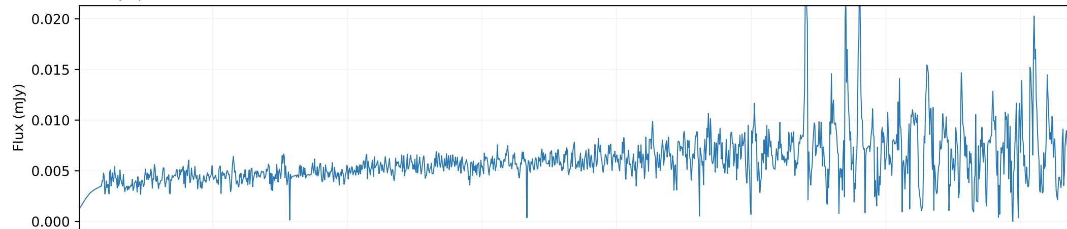
QSO spectrum × 0.0003
