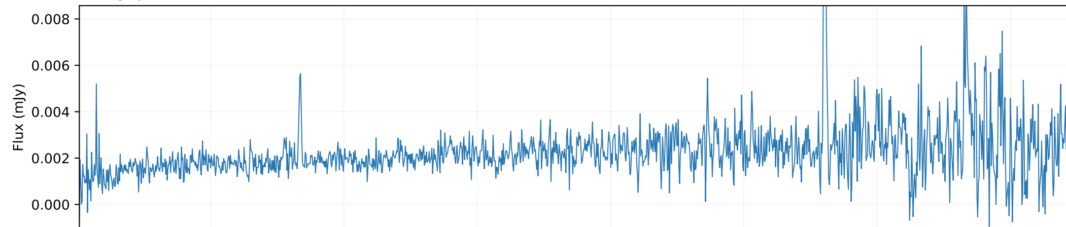
QSO spectrum \times 0.003
