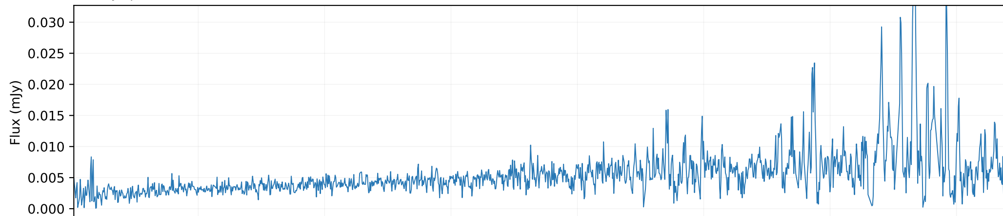
QSO spectrum × 0.0003
