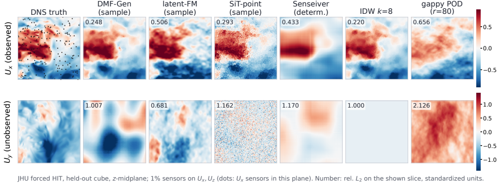
FIG. 4. 3D turbulence, held-out cutout, z-midplane of single reconstructions from 1% sensors on U_x, U_z (identical sensor set throughout; dots mark in-plane sensors). Top row: an observed channel, where every route is competitive. Bottom row: the unobserved U_y , where the fleet-wide identifiability limit is visible — interpolation returns the training mean, gappy POD extrapolates away from the truth, the point-token sampler emits chunk-incoherent noise, and only decoders imposing global field structure produce plausible (if uncorrelated) fields.
