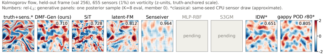
FIG. 3. Kolmogorov flow, held-out trajectory, single reconstructions of vorticity from 655 scattered sensors (1%), identical sensor set for every panel. Architectural signatures are directly legible: the patch tokenizer’s block structure, the latent decoder’s uniform high-frequency texture, the deterministic learner’s smoothing, and the interpolants’ sensor-centred artifacts.
