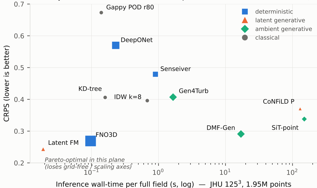
Accuracy vs inference cost (marker area = peak inference GB where measured)
