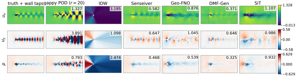
FIG. 3. Surface-only sensing on the held-out Re = 250 frame (128 taps per field, black dots on the body); everything off the body is inferred. Per-panel numbers are single-sample relative L_2 per field. Read against Fig. 2, the identical frame sensed in the volume: gappy POD, which wins there, is beaten several-fold here, and interpolation is worse than the training mean.
