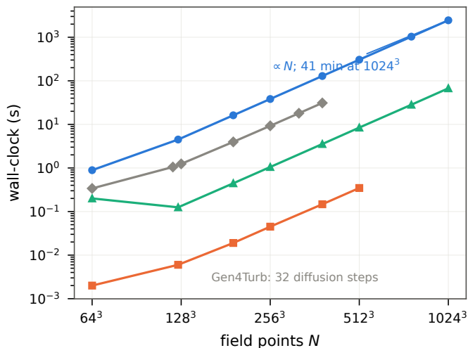
(c) inference — wall-clock per sample
