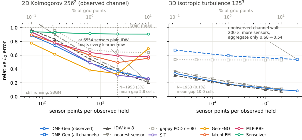
FIG. 6. Reconstruction error versus the number of sensor points, in 2D (left, Kolmogorov 256^2 , the full learned fleet) and 3D (right, JHU 125^3 cross-cube; solid = observed-channel \text{rel-}L_2 , dashed = aggregate over all four channels). Colored = learned; gray = classical floors. The two panels sit on opposite sides of the density story: the same sensor count that leaves a 5.8-cell mean gap in 2D leaves a 10-cell gap in 3D, and while every 3D observed-channel error falls steadily with sensor count — DMF-Gen tracking the interpolation slope from 0.33 to 0.09 over 200\times — the 3D aggregate saturates near 0.54 because the unobserved channels do not identify (Sec. VB). Gappy POD is flat at every 3D density: isotropic turbulence has no low-rank structure for added sensors to project onto. In 2D the fleet fans out rather than sharing a slope: four rows fall monotonically, Geo-FNO and latent FM degrade past \sim 2000 sensors, and Senseiver is nearly flat throughout. Learned rows: canonical protocol, 50 held-out frames, K as in Table V; classical curves: same seeded sensor draws. S3GM’s sweep is still running.
