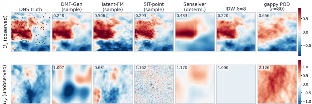
JHU forced HIT, held-out cube, z-midplane; 1% sensors on U_x, U_z (dots: U_x sensors in this plane). Number: rel. L_2 on the shown slice, standardized units.
