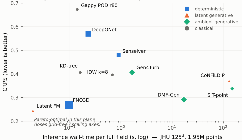
Accuracy vs inference cost (marker area = peak inference GB where measured)
