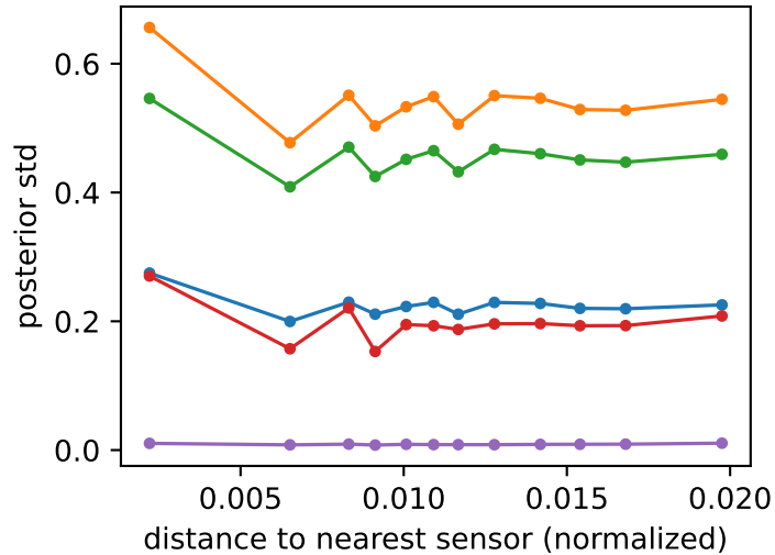
Uncertainty vs sensor distance
