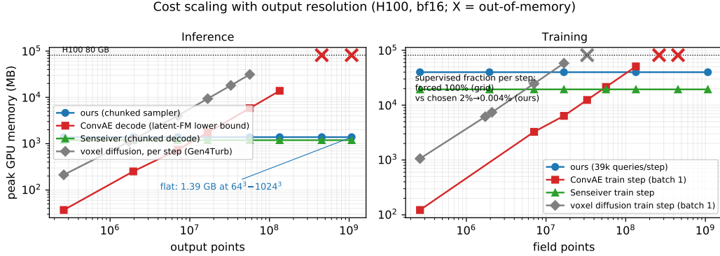
Figure 3: Measured peak memory versus output resolution (H100, bf16, log-log; OOM markers are measured failures, not extrapolations), for full-field sampling (left) and training steps (right). Grid methods (voxel diffusion, convolutional AE) scale cubically and fail at 320^3 and 640^3 ; point methods (LOCUS, Senseiver) are flat to 1024^3 ( 10^9 points). The annotation gives the fraction of the field supervised per training step: 100% forced for grid methods, a fixed 39k-point budget for LOCUS (2% at 125^3 , 0.004% at 1024^3 ). Wall-clock panels are in Figure 5.
