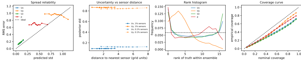
Figure 6: Pointwise uncertainty diagnostics on the held-out cube. Spread reliability: binned RMS error against predicted standard deviation, ideal on the diagonal; the curves are monotone but above it, the pointwise signature of underdispersion. Sensor distance: the profile is flat at 1% coverage and remains flat at 0.1%, where nearest-sensor distances reach eight cells—spread is set by channel identity and flow structure, not by distance to the nearest reading. Rank histogram: U-shaped for the observed channels (underdispersed) and sloped for U_y (biased, as expected for a channel no sensor constrains). Coverage curve: empirical against nominal central-interval coverage.
