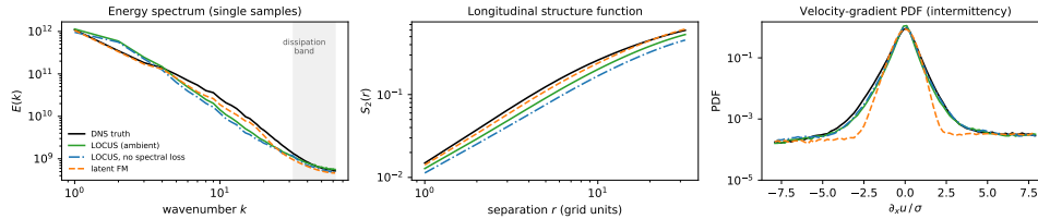
Figure 4: Turbulence statistics of single posterior samples on the held-out region (4 snapshots, NFE 4; ensemble means are deliberately not shown—averaging destroys small scales by construction). Left: shell-averaged energy spectra; the latent baseline carries more inertial-range energy, but truncates in the dissipation band (shaded), where LOCUS tracks the DNS. Middle: longitudinal second-order structure functions. Right: velocity-gradient PDFs, where the latent baseline distorts the shoulders while both LOCUS variants track the DNS shape.
