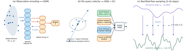
Figure 1: The LOCUS architecture. Sensor tokens are compressed by cross-attention into a small latent array (global pathway, \mathcal{O}(SM) ), which re-injects context back into the sensor tokens. Each query assembles its velocity from its point features, a readout from the latent array, and an importance-weighted retrieval over its K nearest sensor tokens (local pathway, \mathcal{O}(NK) ). No dense volumetric representation is formed; cost is linear in the number of queries, and training estimates the loss on a random \sim 2\% point subset per step.
