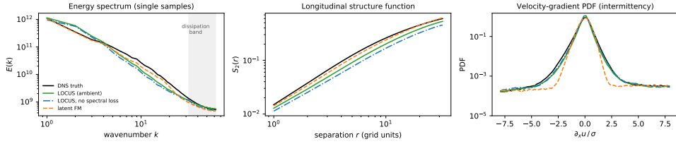
Figure 2: Turbulence statistics of single posterior samples on the held-out region (4 snapshots, NFE 4; ensemble means are deliberately not shown—averaging destroys small scales by construction). Left: shell-averaged energy spectra; the latent baseline carries more inertial-range energy, but truncates in the dissipation band (shaded), where LOCUS tracks the DNS. Middle: longitudinal second-order structure functions. Right: velocity-gradient PDFs, where the latent baseline distorts the shoulders while both LOCUS variants track the DNS shape.
