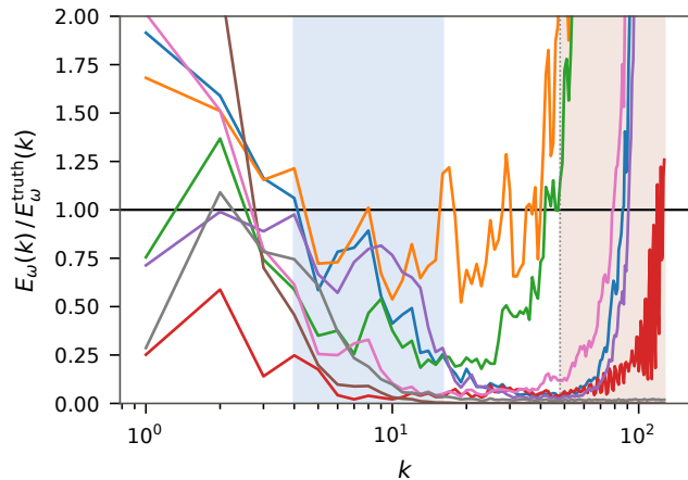
Kolmogorov 256^2 , canonical frame (val 256), 655 vorticity sensors; one posterior sample per generative method. Shaded: energy-carrying inertial (blue) and small-scale (red) bands. Beyond the dotted line the true spectrum holds <0.1\% of peak energy, so ratios there measure spurious energy, not fidelity.
