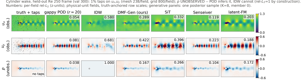
FIG. 2. Cylinder wake, held-out Re = 250 frame, volume sensing: 1% of mesh cells on u_x, u_y (black), p never observed. Single posterior samples, not ensemble means. The p row is the point: gappy POD infers the unobserved channel through the basis’s cross-channel correlations, while interpolation returns the training mean by construction.
