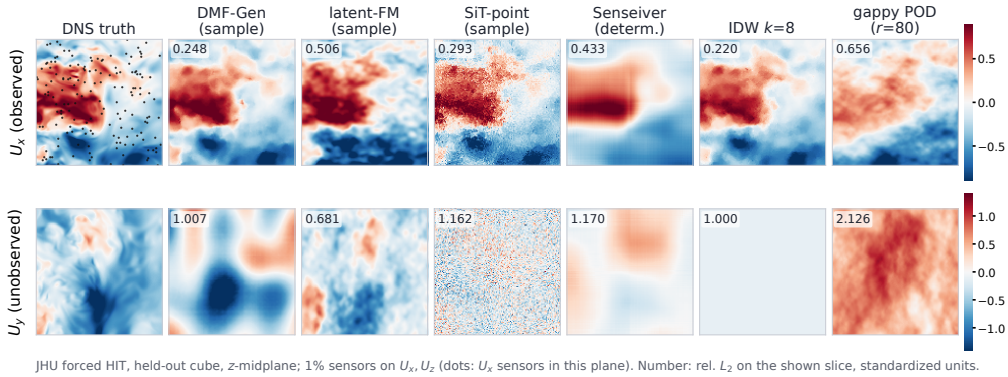
FIG. 5. 3D isotropic turbulence, held-out cutout, z mid-slice: U_x, U_z observed at 1%, U_y and p never observed. Single posterior samples. The unobserved rows are the identifiability wall of Sec. V B: every method produces plausible texture with no pointwise agreement.
