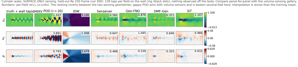
FIG. 3. Surface-only sensing on the held-out Re = 250 frame: taps (black) sit on the body, everything else is inferred. Read against Fig. 2, the identical frame sensed in the volume.
