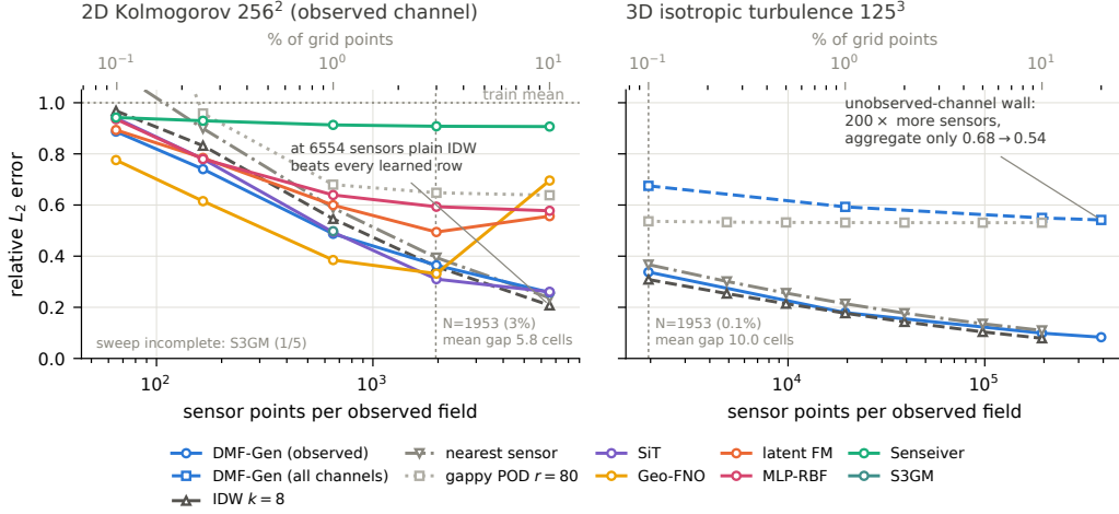
FIG. 6. Reconstruction error versus the number of sensor points, in 2D (left, Kolmogorov 256^2 , the full learned fleet) and 3D (right, JHU 125^3 cross-cube; solid = observed-channel \text{rel-}L_2 , dashed = aggregate over all four channels). Colored = learned; gray = classical floors. The two panels sit on opposite sides of the density story: the same sensor count that leaves a 5.8-cell mean gap in 2D leaves a 10-cell gap in 3D, and while every 3D observed-channel error falls steadily with sensor count — DMF-Gen tracking the interpolation slope from 0.33 to 0.09 over 200\times — the 3D aggregate saturates near 0.54 because the unobserved channels do not identify (Sec. VB). Gappy POD is flat at every 3D density: isotropic turbulence has no low-rank structure for added sensors to project onto. In 2D the fleet fans out rather than sharing a slope: four rows fall monotonically, Geo-FNO and latent FM degrade past \sim 2000 sensors, and Senseiver is nearly flat throughout. Learned rows: canonical protocol, 50 held-out frames, K as in Table VI; classical curves: same seeded sensor draws. S3GM’s sweep is still running.
