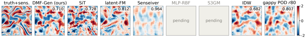
Kolmogorov flow, held-out frame (val 256), 655 sensors (1%) on vorticity (z-units, truth-anchored scale). Numbers: rel- L_2 ; generative panels: one posterior sample ( K=8 eval, member 0).
