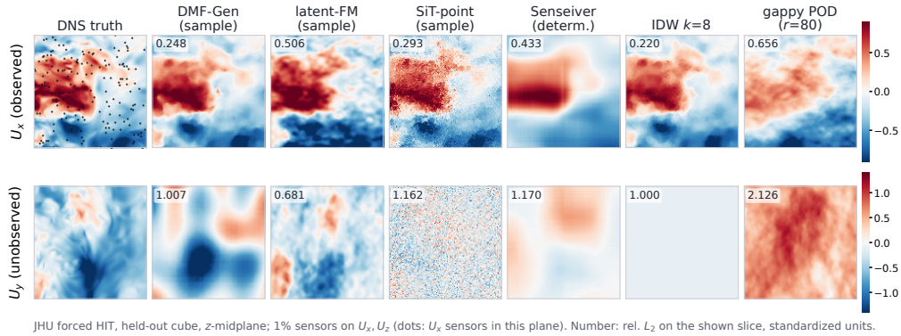
FIG. 5. 3D turbulence, held-out cutout, z-midplane of single reconstructions from 1% sensors on U_x, U_z (identical sensor set throughout; dots mark in-plane sensors). Top row: an observed channel, where every route is competitive. Bottom row: the unobserved U_y , where the fleet-wide identifiability limit is visible — interpolation returns the training mean, gappy POD extrapolates away from the truth, the point-token sampler emits chunk-incoherent noise, and only decoders imposing global field structure produce plausible (if uncorrelated) fields.
