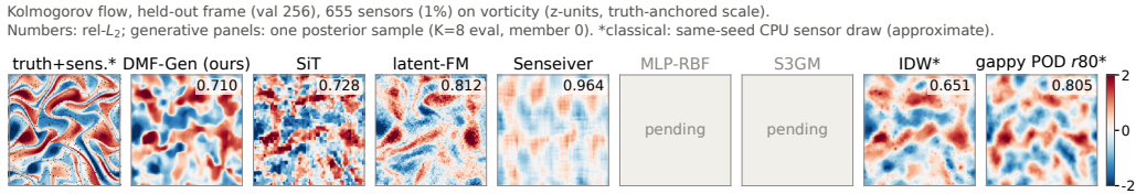
FIG. 4. Kolmogorov flow, held-out trajectory, single reconstructions of vorticity from 655 scattered sensors (1%), identical sensor set for every panel. Architectural signatures are directly legible: the patch tokenizer’s block structure, the latent decoder’s uniform high-frequency texture, the deterministic learner’s smoothing, and the interpolants’ sensor-centred artifacts.
