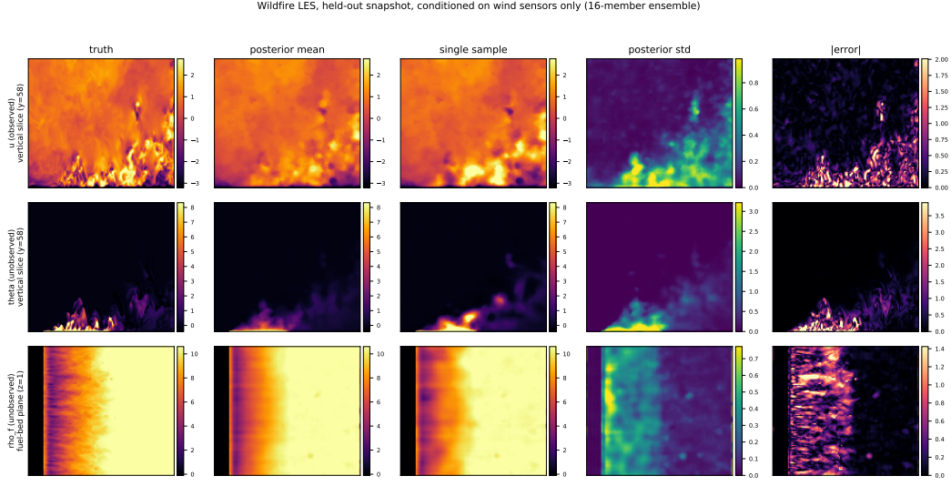
Figure 7: Wildfire LES, held-out snapshot, conditioned on wind sensors only. Wind and potential temperature are shown on a vertical slice through the plume; fuel density is shown on the fuel-bed plane, where its structure lives. Potential temperature and fuel density are never observed. From wind alone the model localizes the burn scar and its ragged front, and the predictive standard deviation concentrates on that front—the reconstruction is confident in the burned and unburned interiors and uncertain exactly where the front sits.
