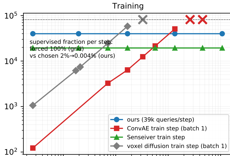
Cost scaling with output resolution (H100, bf16; X = out-of-memory)
