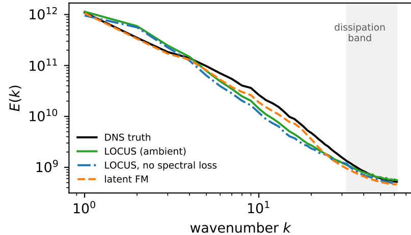
Energy spectrum (single samples)
