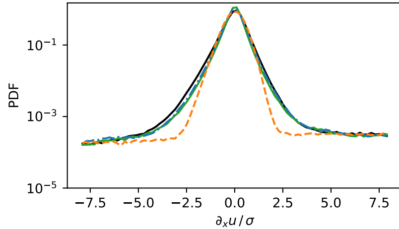
Velocity-gradient PDF (intermittency)
