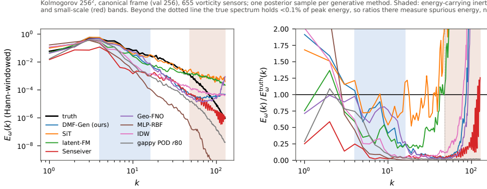
FIG. 7. Kolmogorov 256 2 shell spectra of single samples on the canonical frame, 655 vorticity sensors, Hann-windowed. Left: spectra against DNS. Right: ratio to truth. Shaded: the energy-carrying inertial band (blue) and the small-scale band (red). Beyond the dotted line the true spectrum holds under 0.1% of its peak, so ratios there measure energy a method invented rather than energy it recovered — which is why we score fidelity on the shaded bands and report the tail separately.
