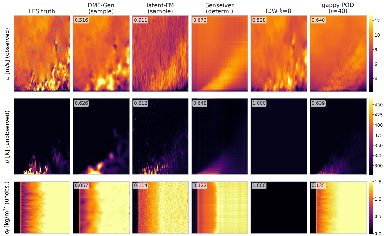
FireBench wildfire LES, held-out frame; wind sensors only (1% on u , v , w ; dots: u sensors in the slice). Rows 1-2: vertical slice y=58 ; row 3: fuel-bed plane z=1 .
