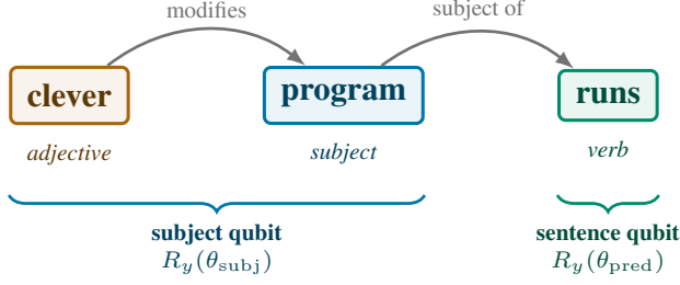
Figure 1. The grammatical parse of an example sentence. Roles, not word order, decide which qubit each word rotates: the subject side (adjective + noun) feeds the subject qubit, the predicate side (verb, and any object) feeds the sentence qubit. These assignments wire the angles into the circuit of Figure 2.
