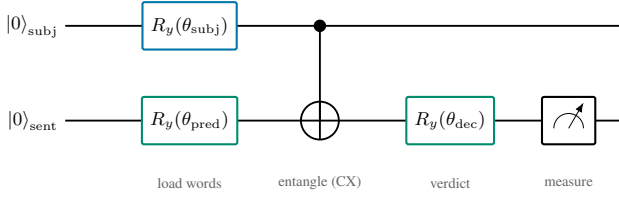
Figure 2. The two-qubit circuit, read left to right. Word parameters set the opening rotations R_y(\theta_{\text{subj}}) and R_y(\theta_{\text{pred}}) . The CX gate (control \bullet on the subject, target \oplus on the sentence) entangles the two qubits, which is grammatical composition. The final decision rotation R_y(\theta_{\text{dec}}) writes in the sentiment verdict before the sentence qubit is measured.
