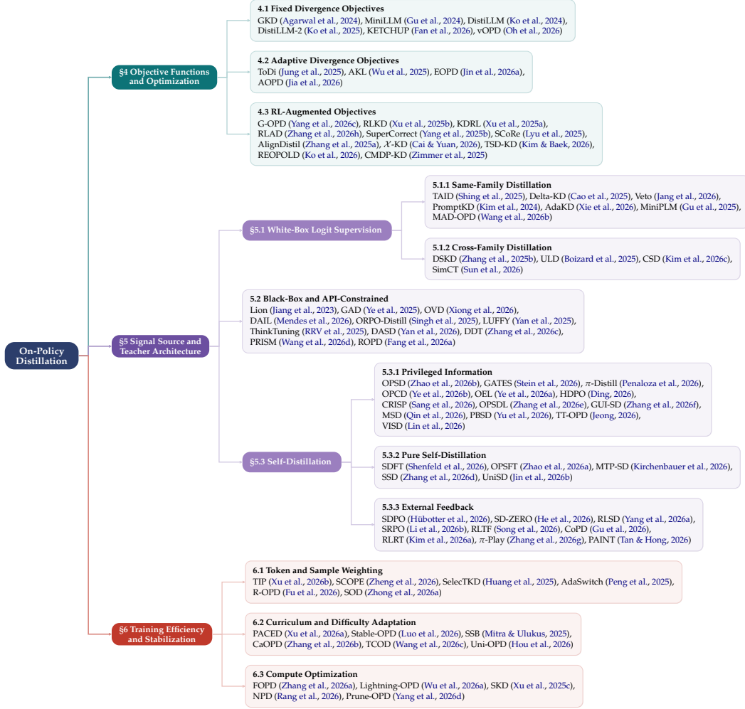
Figure 1: Taxonomy of On-Policy Distillation methods organized along three design axes: (1) Objective function design (§4), (2) Signal source and teacher architecture (§5), and (3) Training dynamics and efficiency (§6). Each leaf lists representative methods with a badge showing the method count. Methods are placed under their primary contribution. Those contributing to secondary dimensions (e.g., PAINT and PRISM contributing implicit curricula) are discussed in the relevant section prose rather than duplicated in the tree.
