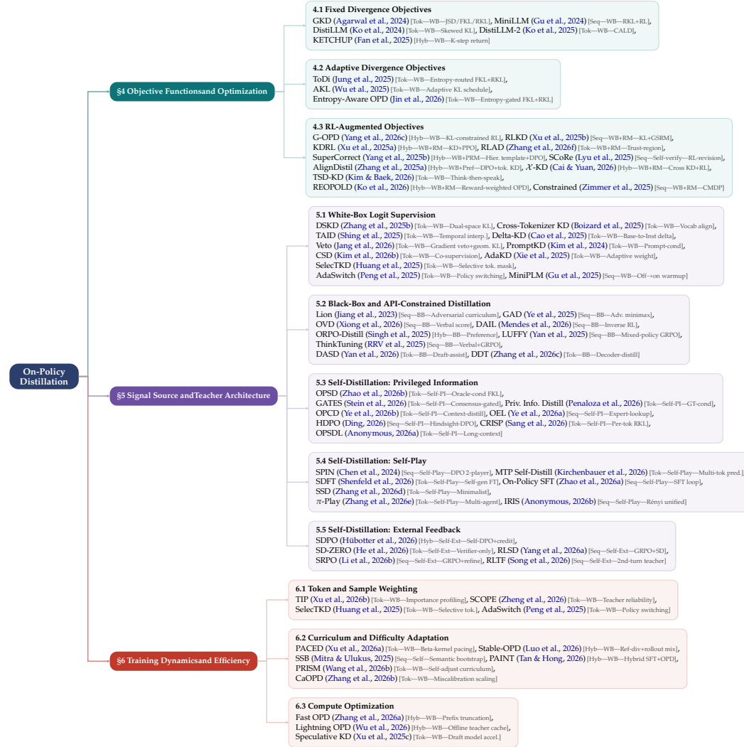
Annotation key. Each method carries a compact three-field tag [Granularity | Signal | Divergence/Loss]. Granularity: Tok = token-level, Seq = sequence-level, Hyb = hybrid. Signal: WB = white-box logits, BB = black-box API, RM = reward model, PRM = process reward model, Pref = preference pairs, Self-PI = privileged information, Self-Play = self vs. reference, Self-Ext = external verifier/reward, Self-verify = self-verification. Divergence/Loss: FKL/RKL = forward/reverse KL, JSD = Jensen-Shannon, CALD = contrastive-approximated likelihood difference, CMDP = constrained MDP, DPO = direct preference optimization, GRPO = group relative policy optimization, PPO = proximal policy optimization. The numeric badge on each leaf gives the method count.
