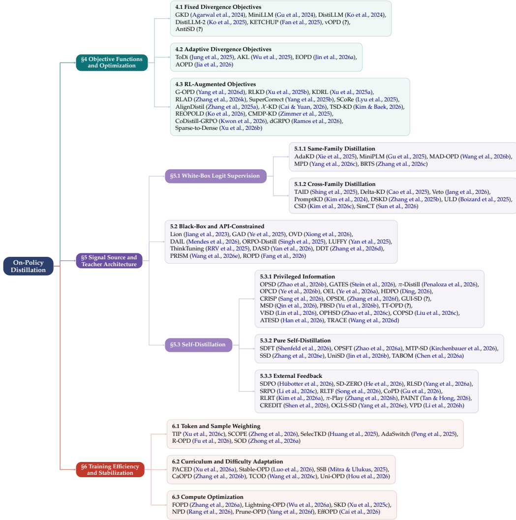
Figure 1: Taxonomy of On-Policy Distillation methods organized along three design axes: (1) Objective function design (§4), (2) Signal source and teacher architecture (§5), and (3) Training dynamics and efficiency (§6). Each leaf lists representative methods with a badge showing the method count. Methods are placed under their primary contribution. Those contributing to secondary dimensions (e.g., PAINT and PRISM contributing implicit curricula) are discussed in the relevant section prose rather than duplicated in the tree.
