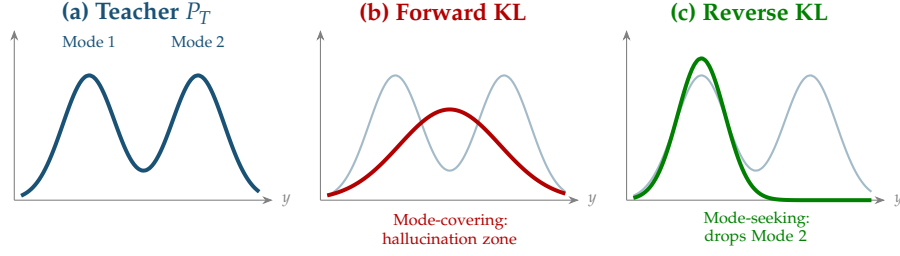
Figure 2: Forward KL vs. Reverse KL for fitting a student distribution P_S to a bimodal teacher P_T . (a) The teacher has two modes. (b) Forward KL is mode-covering (zero-avoiding): the student covers both modes but places mass in the inter-mode hallucination zone. (c) Reverse KL is mode-seeking (zero-forcing): the student concentrates on a single mode, dropping the other entirely. Adaptive methods (ToDi, AKL) dynamically switch between the two based on local distributional geometry.
