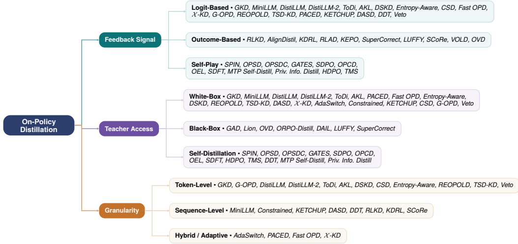
Figure 2: Taxonomy of on-policy distillation for large language models. The methodology space is organized along three orthogonal dimensions with representative methods. A single method may appear across multiple categories as these axes are independent.
