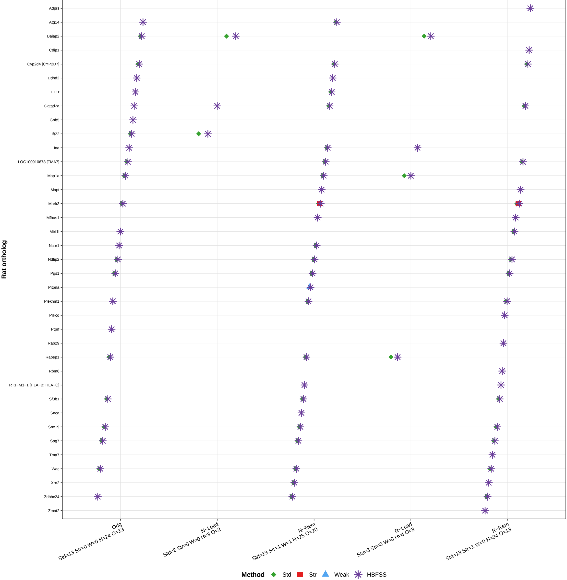
RT4_ZT10 | 3'aTwas ortholog overlap Significant WTTs ortholog genes across five analysis views | genes=37
