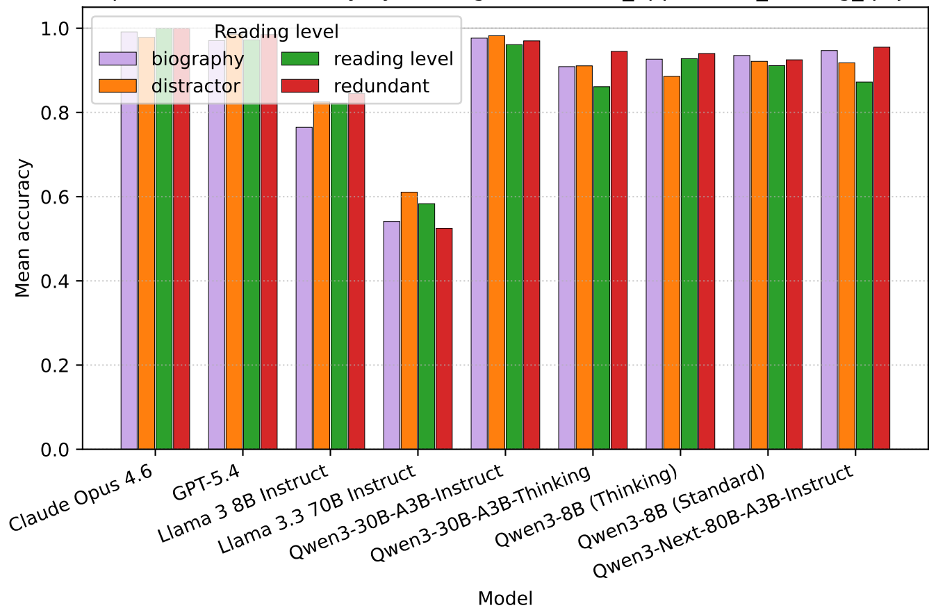
Compactor mean accuracy by reading level — wm_application_reading_qa.json
