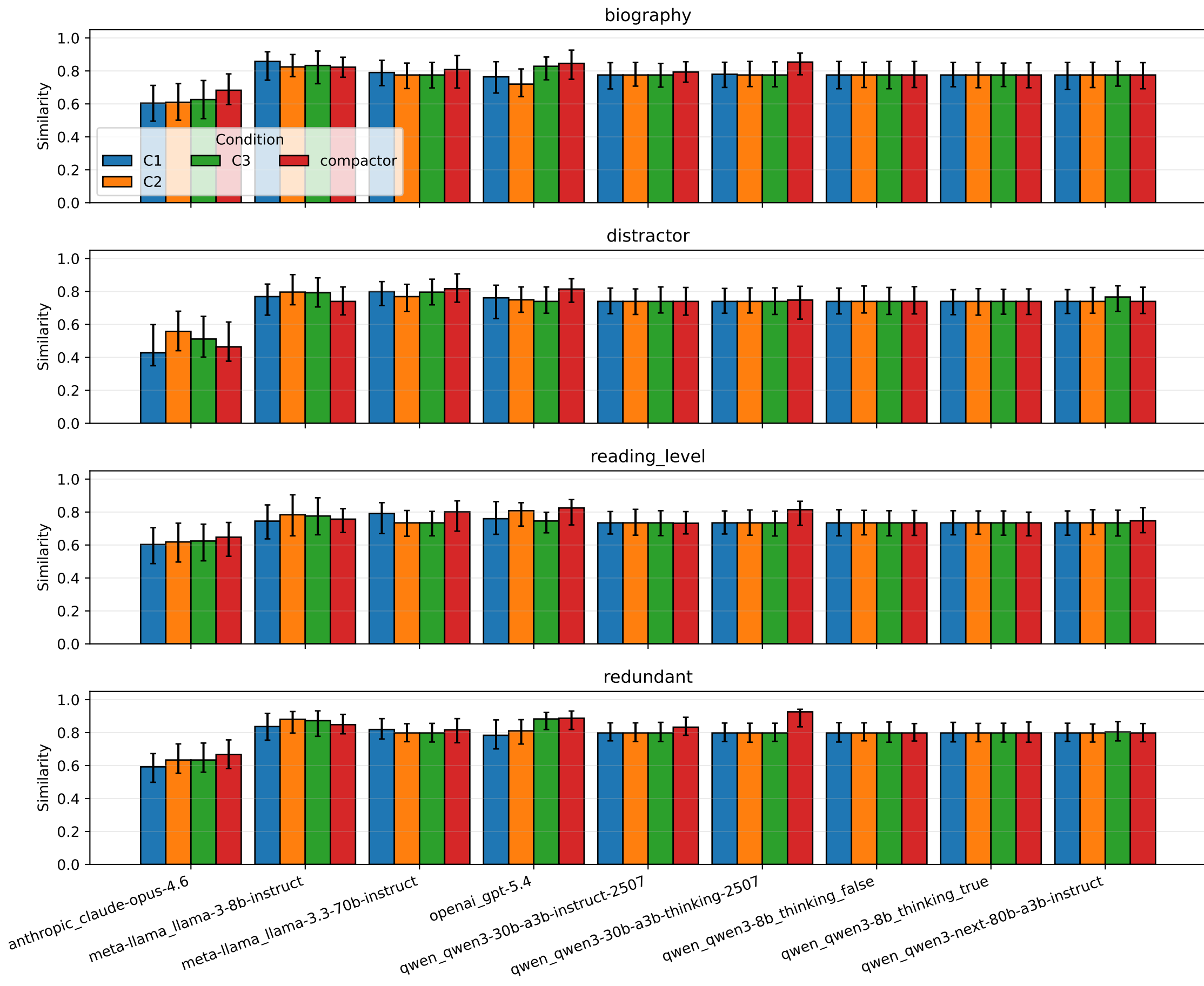
Difficulty similarity | x=model, grouped/color=condition, subplots=level
