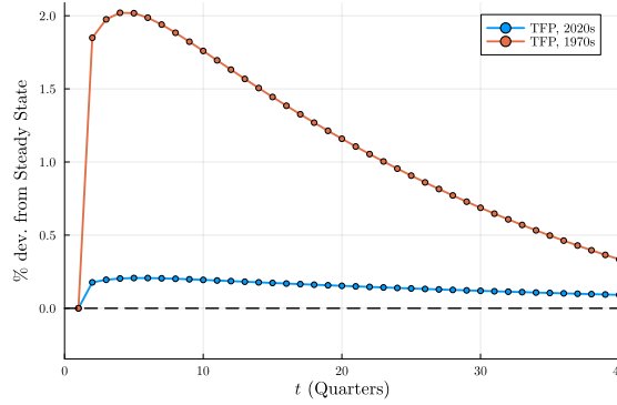
(a) Productivity (TFP) Impulse Responses, 1970 and 2022
