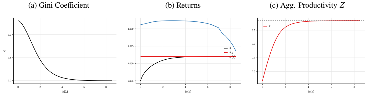
Figure 4: Steady State Comparative Statics in \sigma_z
