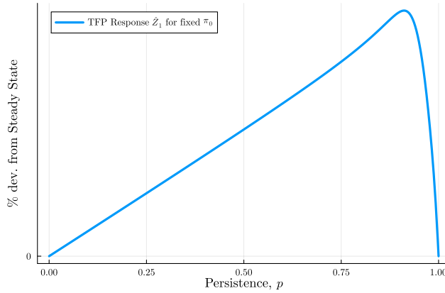
Figure 7: Productivity Response \hat{Z}_1 (fixed \pi_0 )
