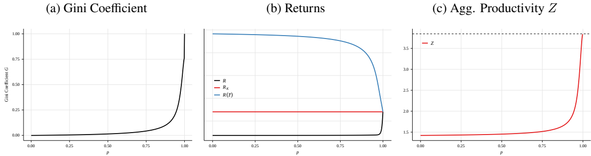
Figure 2: Steady State Comparative Statics in p
