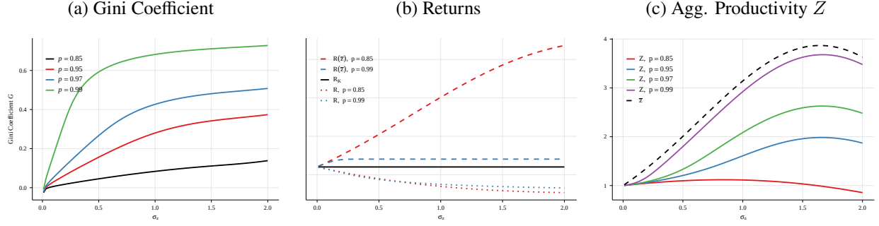
Figure 3: Steady State Comparative Statics in \sigma_z
