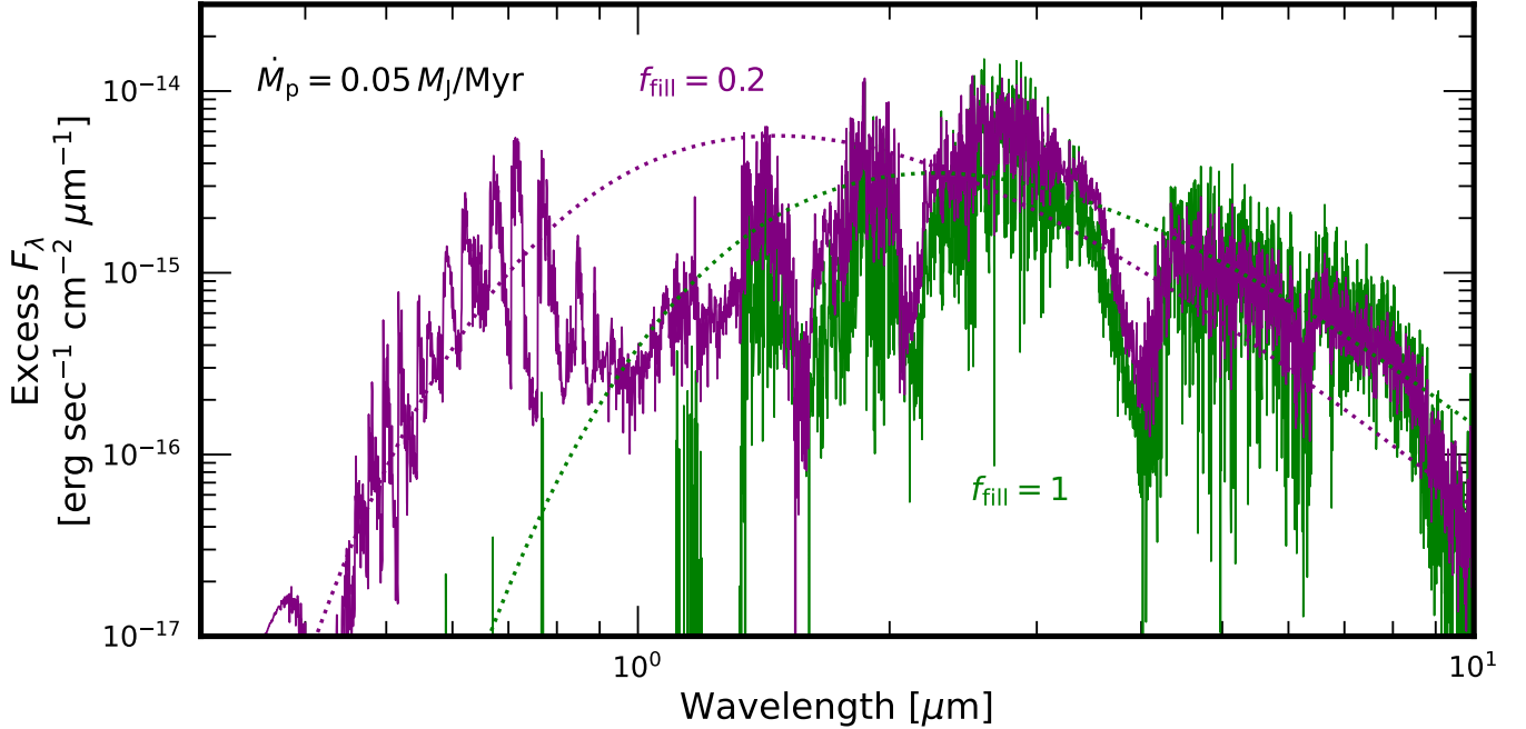
Figure 5. Effect of accretion geometry on a protoplanet’s spectrum. The y -axis plots the excess flux relative to the undisturbed atmosphere. The green curve shows the case where the planet accretes in a spherically symmetric manner at a rate \dot{M}_p = 0.05 M_J/\text{Myr} . The purple curve shows a case with the same \dot{M}_p , but now assuming accretion only happens over a fraction f_{\text{fill}} = 0.2 of the planet’s surface. The resulting excess spectrum arises from a combination of accretional hotspots dominating the emission at short wavelengths plus a redder non-accreting component. Dotted lines indicate approximate excesses that would be expected if the accreting regions radiated as dilute blackbodies.
