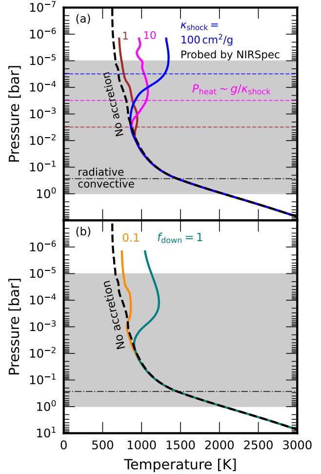
Figure 4. Similar to Fig. 1a, but now showing how the atmosphere responds to changes in model parameters at fixed \dot{M}_{\text{p}} = 0.01 M_{\text{J}}/\text{Myr} . The top panel varies the atmosphere's opacity to shock radiation \kappa_{\text{shock}} . Larger values concentrate the accretional energy into a narrower layer. Dashed lines mark an order-of-magnitude estimate for the depth of the heated layer. The bottom panel varies f_{\text{down}} , the fraction of accretion power that contributes to atmospheric heating.
